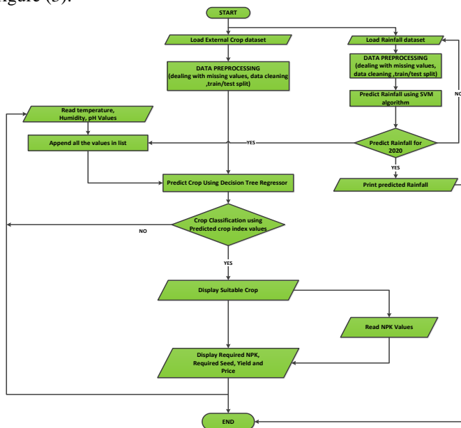
Figure 3. Proposed System Flow chart.
