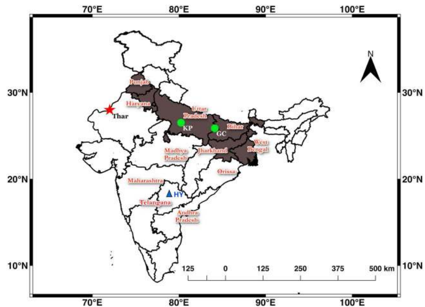
Figure 1. Map showing the study area and different states mentioned in the text. The green circles show locations of two AEROSOL ROBOTIC NETWORK stations (KP = Kanpur and GC = Gandhi College). The region shaded in dark gray represents the Indo-Gangetic Basin. The location of the Thar Desert (one of the largest dust source regions in India) has been shown with a red star. City of Hyderabad (HY) has been marked with a blue triangle.
