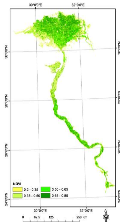
Figure 3. NDVI distribution.
