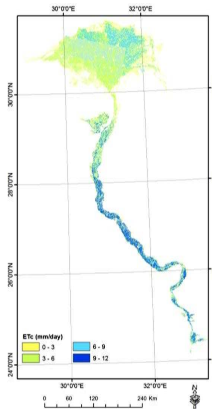
Figure 4. Kc distribution..
