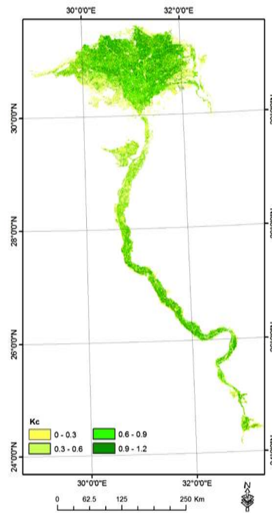
Figure 4. Kc distribution..
