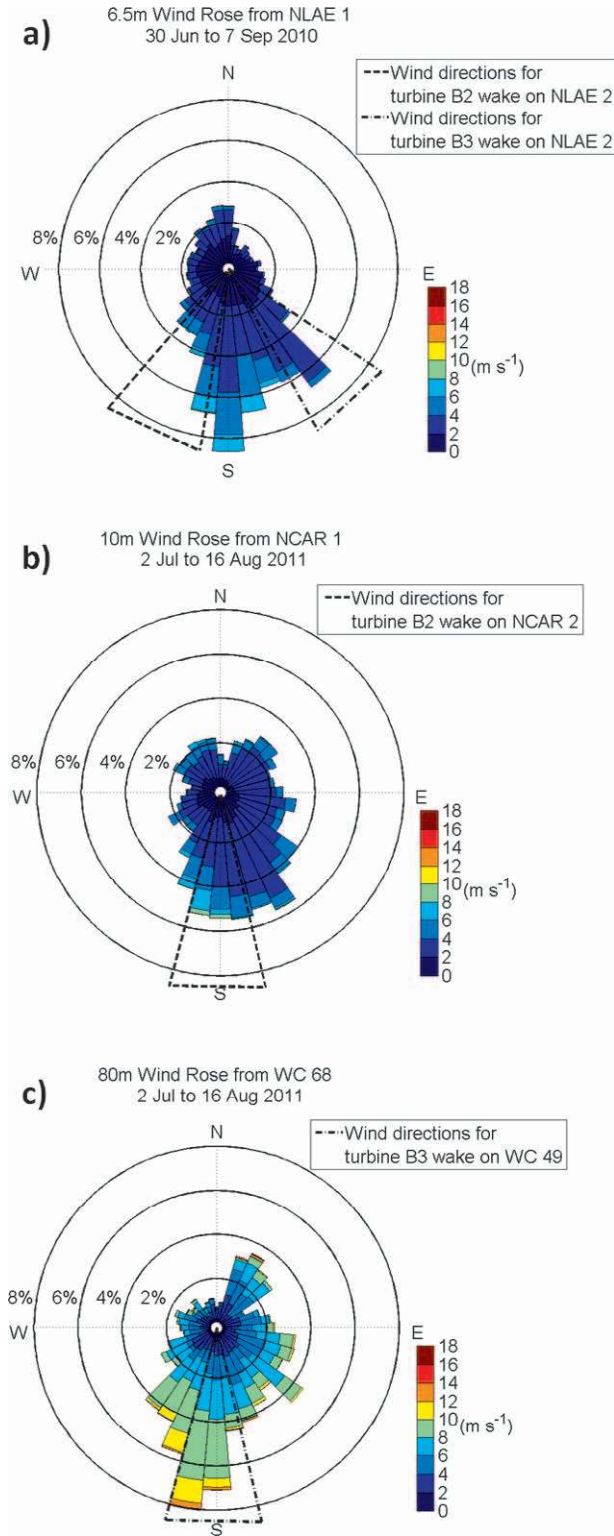
FIG. 3. Wind roses for (a) CWEX-10 6.5-m winds at the reference flux tower (NLA E 1), (b) CWEX-11 10-m winds at the reference flux tower (NCAR 1), and (c) CWEX-11 80-m winds from the upwind Windcube (WC 68). Dashed lines denote wind directions for turbine wakes on downwind stations.
