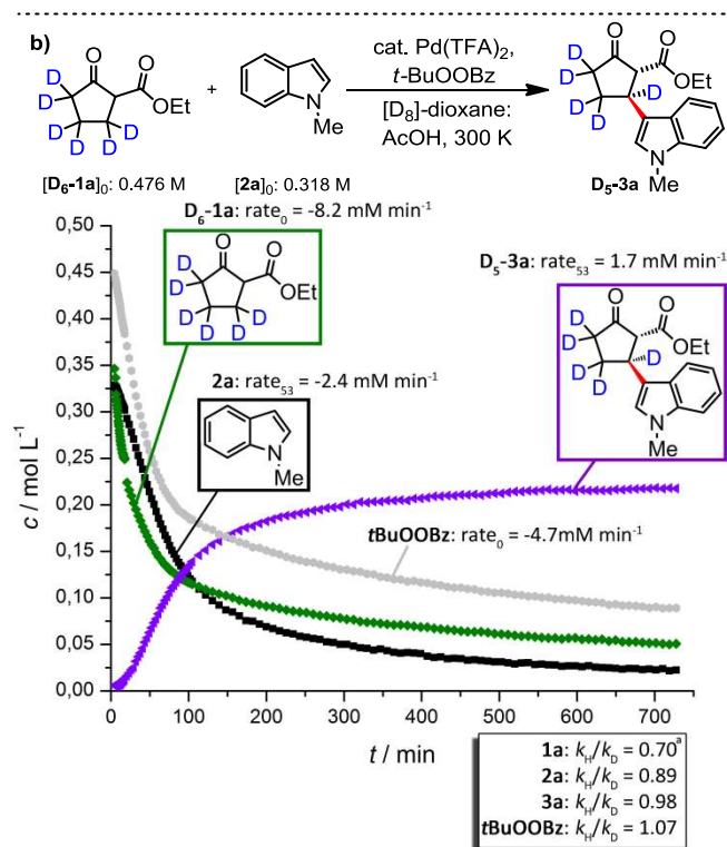
Figure 2. Temporal progress of the coupling by ^1\text{H} NMR spectroscopy with deuterated starting materials. Reaction conditions: a) [\mathbf{1a}]_0 = 0.476 \text{ M} , [\mathbf{D-2a}]_0 = 0.318 \text{ M} , b) [\mathbf{D}_6\text{-1a}]_0 = 0.476 \text{ M} , [\mathbf{2a}]_0 = 0.318 \text{ M} . For both experiments: [\text{tBuOOBz}]_0 = 0.413 \text{ M} , 10 mol% \text{Pd}(\text{TFA})_2 , 4:1 [\text{D}_8]\text{-Dioxane}/\text{AcOH} , 300 K. Rates and k_H/k_D are averages of three experiments (a) or two experiments (b). \text{rate}_0 and \text{rate}_{xx} refer to the initial rate and the rate at t = xx min, respectively.
