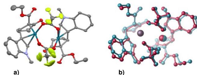
Figure 9. Structure of the Pd 2 (TFA) 2 ( 3a ) 2 complex: a) X-ray structure, b) overlay of X-ray (blue) and computed (red) structures.
