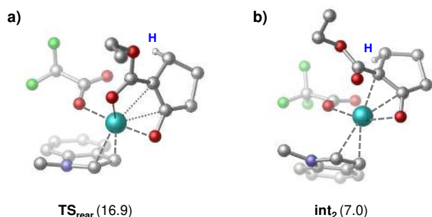
Figure 4. Decoordination of the ester group in intermediate int 1 : a) transition state, b) product state of rearrangement.
