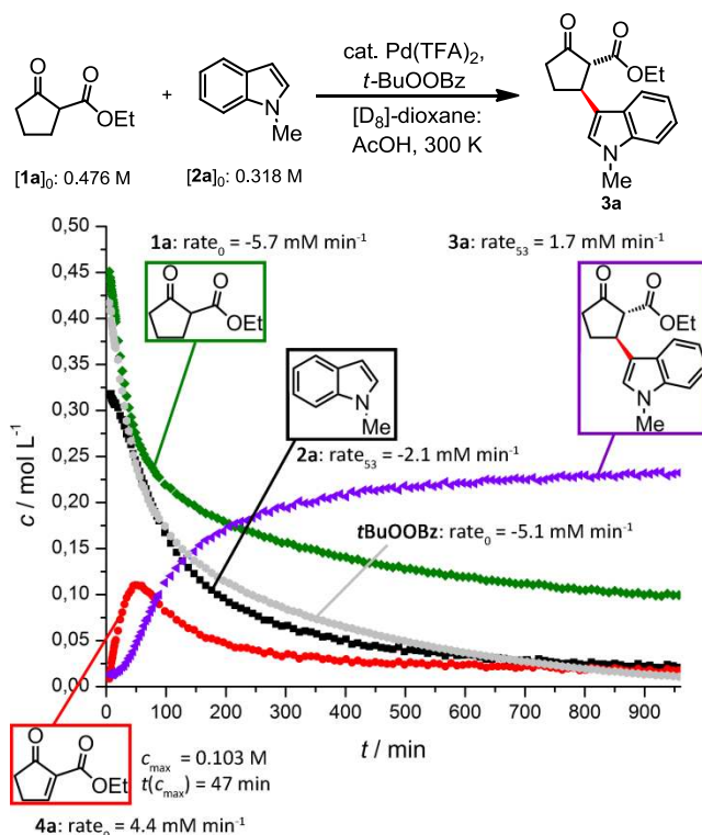
Figure 1. Monitoring of the temporal progress of the coupling by 1 H NMR spectroscopy. Reaction conditions: [ 1a ] 0 = 0.476 M, [ 2a ] 0 = 0.318 M, [ t BuOOBz] 0 = 0.413 M, 10 mol% Pd(TFA) 2 , 4:1 [D 8 ]-dioxane/AcOH, 300 K. The reported rates are averages of three experiments. Rate 0 and rate 53 refer to the initial rate and the rate at t = 53 min, respectively.
