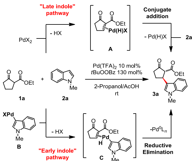
Figure 1. Monitoring of the temporal progress of the coupling by 1 H NMR spectroscopy. Reaction conditions: [ 1a ] 0 = 0.476 M, [ 2a ] 0 = 0.318 M, [ t BuOOBz] 0 = 0.413 M, 10 mol% Pd(TFA) 2 , 4:1 [D 8 ]-dioxane/AcOH, 300 K. The reported rates are averages of three experiments. Rate 0 and rate 53 refer to the initial rate and the rate at t = 53 min, respectively.
