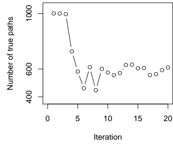
Fig. 4. Convergence of number of paths satisfying \diamond D \geq 470 in the chemical model using N_j = 1000 .
