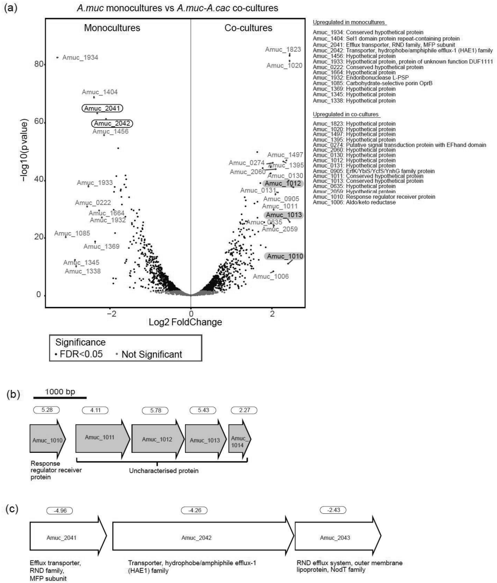
Figure 3. (a) Volcano plots showing p-values correlated to fold changes in gene expression of Akkermansia muciniphila observed in monocultures versus co-cultures with Anaerostipes caccae . Positive fold changes indicate upregulation in co-cultures, and negative fold changes indicate upregulation in monocultures. Locus tags for genes with Log2 fold change >2 (or fold change >4) are labelled. (b) Response regulator and putative operon upregulated in the co-cultures (c) Putative operon upregulated in the monocultures. Fold changes are listed above the respective genes.
