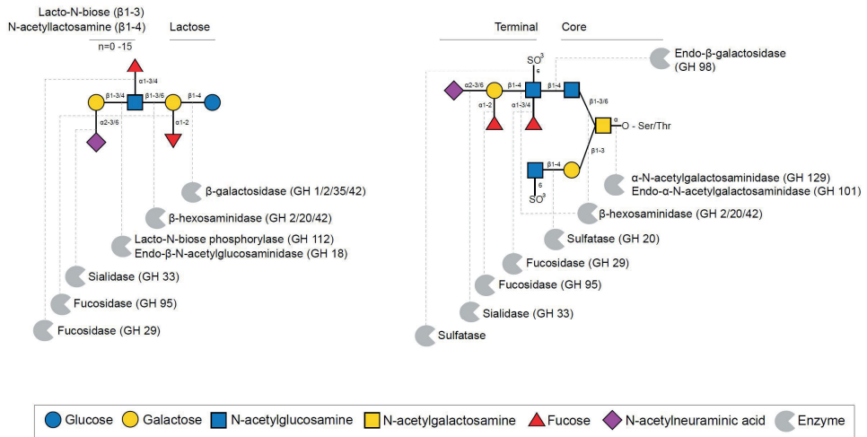
Figure 1. The structure of HMOS and mucins show molecular similarities. The schematic representation for (A) HMOS and (B) mucin O-glycans, summarising the sites of action and carbohydrate-active enzymes (CAZymes) (Lombard et al 2014) predicted to cleave the glycosidic linkages. N-acetylneuraminic acid (Neu5Ac), the predominant sialic acid in mammalian cells is depicted. HMOS may also carry \alpha 1-2 fucose linked to galactose, \alpha 1-3 fucose linked to glucose, and/or \alpha 2-6 Neu5Ac linked to GlcNAc. The depiction for specific HMOS structures are available at Thurl et al. (Thurl et al 2017). The hypothetical mucin O-glycan chain is adapted from Tailford et al. (Tailford et al 2015). Detailed structural representation for mucin O-glycans is available at Brockhausen and Stanley (Brockhausen and Stanley 2017). Abbreviation: GH, glycosyl hydrolase.
