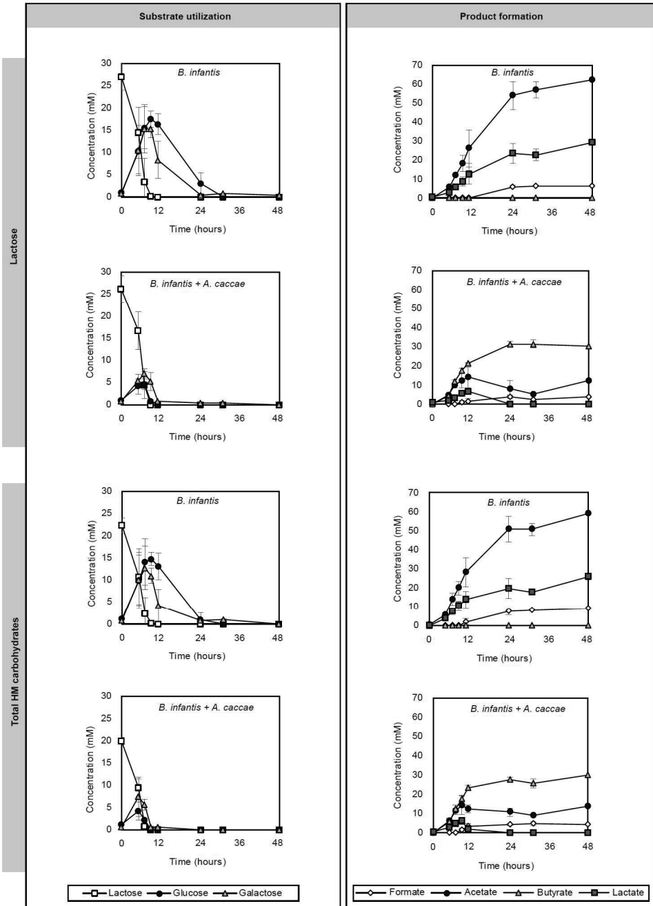
Figure 3. Bifidobacterium infantis supported butyrate production of Anaerostipes caccae . The substrate utilisation and SCFA formation of co-cultures in lactose or total HM carbohydrates. Error bars represent the standard deviation for biological triplicates, except for time point 31 h (n=2) and 48 h (n=1).
