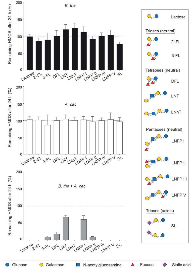
Figure 3. Utilisation of HMOS structures by Bacteroides thetaiotaomicron and Anaerostipes caccae co-culture. No HMOS degradation was detected for the monoculture of Bacteroides thetaiotaomicron and Anaerostipes caccae after 24 h of fermentation. The HMOS structures and glycosidic linkages are depicted according to Varki et al. (Varki et al. 2015). Error bars represent the error propagation for mean of two biological replicates measured in technical triplicates. Abbreviations: 2'-FL, 2'-fucosyllactose; 3-FL, 3-fucosyllactose; DFL, difucosyllactose; LNT, lacto-N-tetraose; LNnT, lacto-N-neotetraose; LNFP I, lacto-N-fucopentaose I; LNFP II, lacto-N-fucopentaose II; LNFP III, lacto-N-fucopentaose III; LNFP V, lacto-N-fucopentaose V; SL, sialyllactose.
