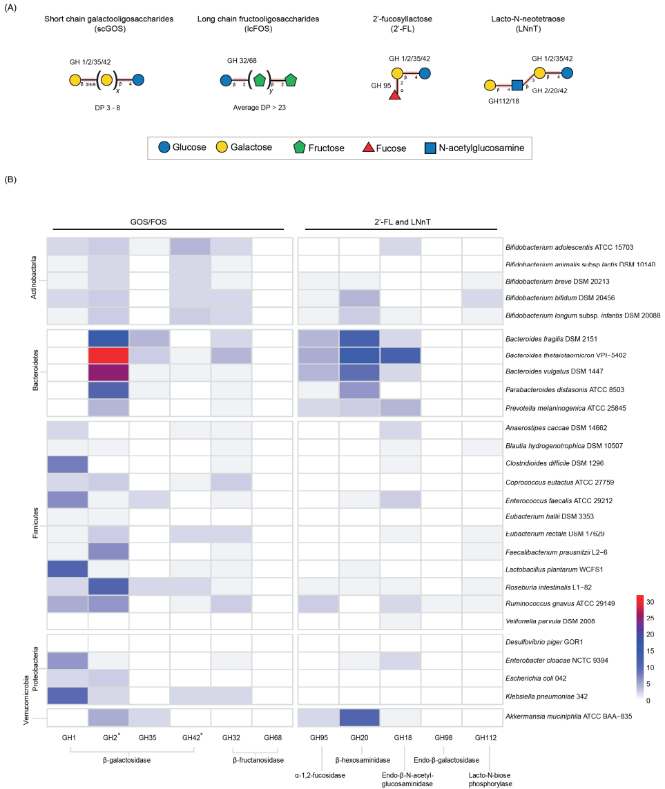
Figure 2. Prebiotics in infant nutrition. (A) The combination of scGOS and lcFOS at 9:1 ratio has been widely supplemented in infant formula whereas HMOS including 2'-FL and LNnT are currently evaluated in clinical study. (B) Prediction for bacterial carbohydrate-active enzymes (CAZymes) involved in the catabolism of prebiotics for the representative species in the human gut. Colour key indicating the number of CAZymes predicted in the genome. Abbreviations: DP, degree of polymerization; GH, glycosyl hydrolase. (*) GH 2 and GH 42 are also predicted for β-hexosaminidase function.
