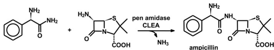
Figure 1 | Ampicillin synthesis
