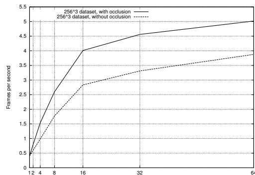
Figure 10: Comparison of performance with and without cross-processor occlusion using the 256^3 head CT dataset.
