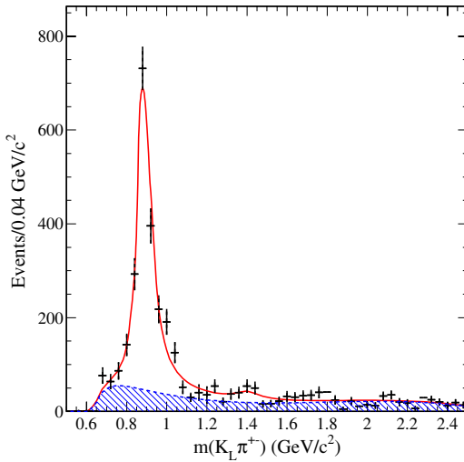
FIG. 23 (color online). The number of K^*(892)^\pm events obtained from fits to the K_S^0 K_L^0 \pi^\pm invariant mass distribution in each 0.04 \text{GeV}/c^2 interval of K_L^0 \pi^\pm mass. The curve represents the result of the fit described in the text, with the hatched areas representing the nonresonant component.
