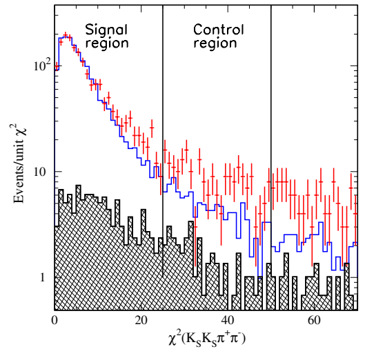
FIG. 25 (color online). The four-constraint \chi^2 distributions for K_S^0 K_S^0 \pi^+ \pi^- \gamma candidate events selected in the data (points) and signal-MC simulation (open histogram) fitted under the K_S^0 K_S^0 \pi^+ \pi^- hypothesis. The cross-hatched histogram represents the simulated background contribution from non-ISR q\bar{q} events.
