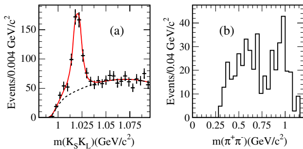
FIG. 24 (color online). (a) The K_S^0 K_L^0 invariant mass distribution for the selected K_S^0 K_L^0 \pi^+ \pi^- events. The solid and dashed lines represent the result of the fit described in the text and its non- \phi component, respectively. (b) The \pi^+ \pi^- invariant mass distribution for events in the \phi peak (see the text).
