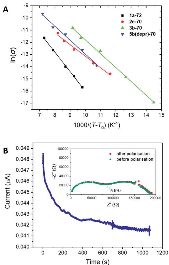
Fig. 4 (A) VTF fitting for selected SPE samples ( T_0 = T_g - 50 K); (B) representative chronoamperometry and Nyquist plot (inlaid) obtained for the determination of t_+ for 2e-70 . A 10 mV applied polarization voltage was used for the chronoamperometry in a symmetrical Li|SPE|Li cell. The Nyquist plot was obtained by EIS recorded in the frequency range of 0.1 Hz to 1 MHz and the annotated frequency corresponds to the resistance at the intersecting circles.
