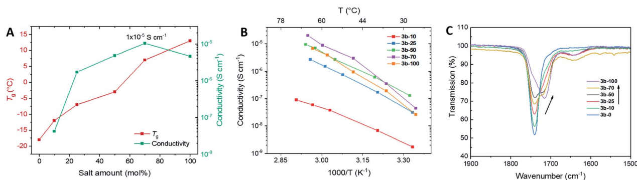
Fig. 3 Characterisation data for SPEs 3b–x ( M_{n,SEC} = 27.4–27.9 kg mol -1 , 0.05 equivalents of EDDT), with varying amount of LiTFSI salt; (A) conductivity (normalised to 60 °C) and T_g as a function of salt molarity; (B) Arrhenius plot showing the temperature dependence of the ionic conductivities of SPEs 3b–x ; (C) Signals in FTIR spectrum representing C=O stretching vibration.
