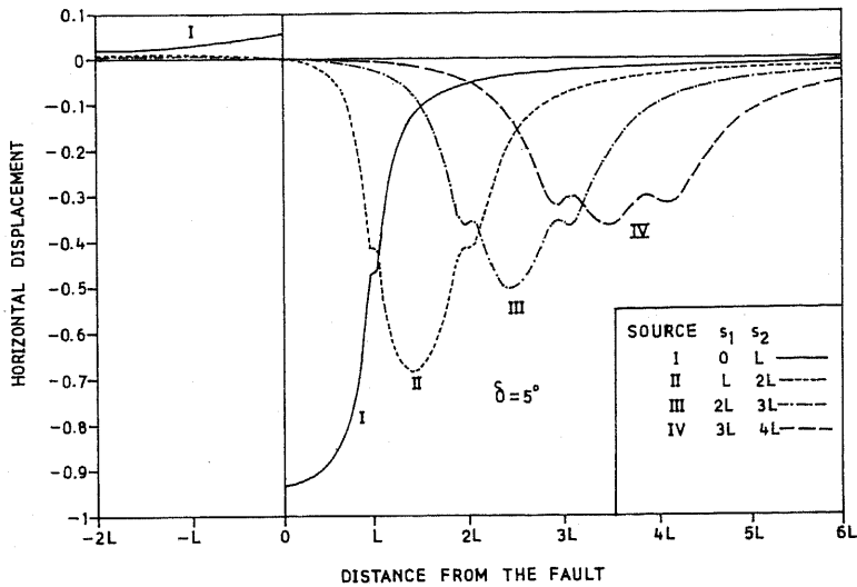
Fig. 2(a). Variation of the dimensionless horizontal displacement ( u_2/b ) with the distance from the fault ( x_2 ) for dip angle \delta=5^\circ .
