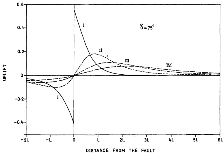
Fig. 3(f). Variation of the uplift with x_2 for \delta = 75^\circ .
