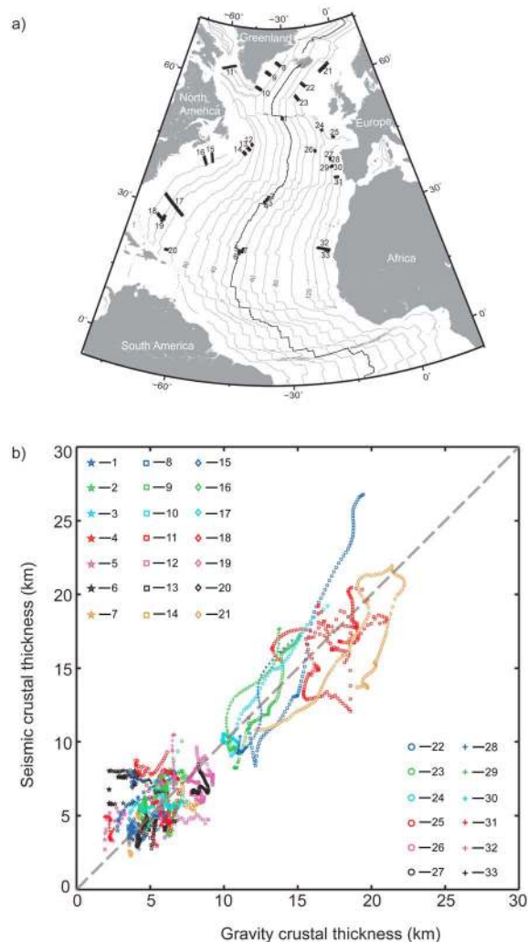
Figure 4. (a) Locations of seismic refraction profiles used for comparison of gravity-derived and seismically determined crustal thickness in Figure 4b. See Figure S3 for comparisons within individual seismic profiles. (b) Comparison of gravity-derived crustal thickness (Figure 5) with seismically determined crustal thickness from 33 seismic refraction profiles in the North Atlantic Ocean. Each point corresponds to a sample every 2 km along the seismic profile. Symbols are identified with profile numbers shown in Figure 4a.
