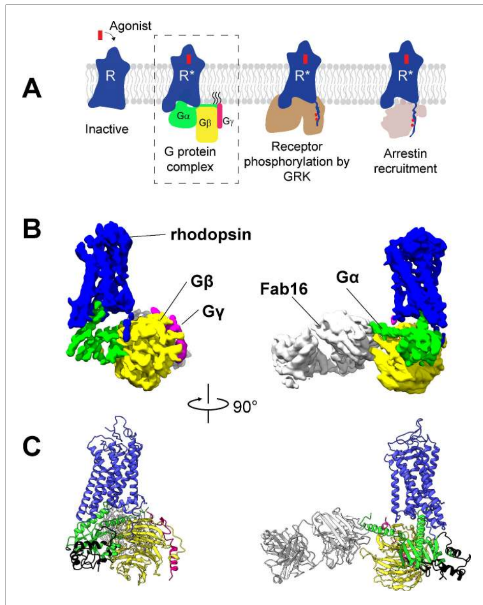
Figure 1. Cryo-EM structure of the rhodopsin-Gi-Fab16 complex. (A) GPCR signaling complexes. (B) EM density map of the complex (rhodopsin – blue, G \alpha i – green, G \beta – yellow, G \gamma – magenta, Fab16 – white). (C) Atomic model of the complex (same color code as B). The region of the Ras domain of G \alpha with no corresponding density in the EM map is depicted in back.
