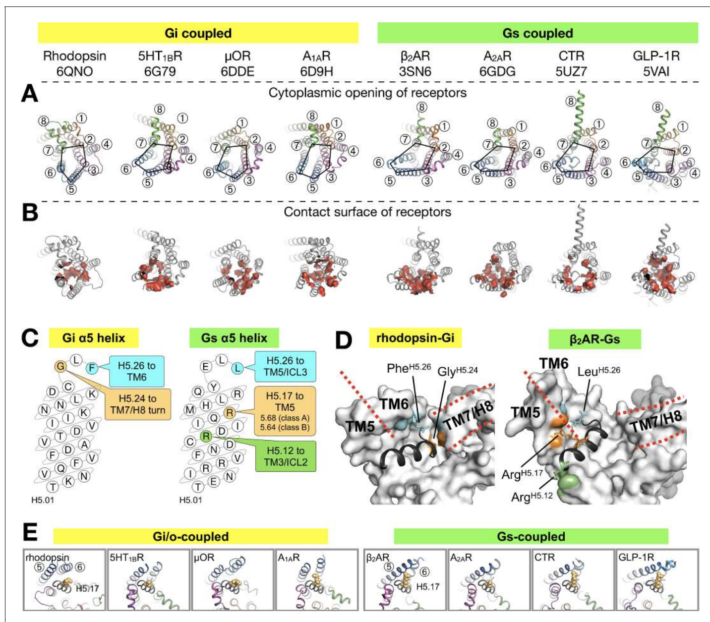
Figure 3. Binding of the G \alpha \alpha 5 helix in GPCR-G protein complexes. (A) Overview of a subset of GPCR-G protein complexes used for this analysis. For a complete list of the complexes used, see Figure 3—figure supplement 2 . The complexes are shown from the cytoplasmic side, and the black pentagons connecting TM2-3-5-6-7 delineate the G protein-binding interface. Receptors are represented in ribbons with their TM helices numbered. (B) The red surfaces depict the contact area (within a distance of 4 Å) between the receptor and the \alpha 5 helix of G \alpha . (C) Schematic representation of the \alpha 5 helix in Gi- and Gs-subtypes. The residues highlighted, and their respective binding site to the receptor, are conserved among all Gi, and Gs, complexes analyzed. All contacts retrieved from this analysis are reported in Figure 3—figure supplement 2 . (D) Position of Gi- and Gs-specific contacts shown in the rhodopsin-Gi (this work, PDB id: 6QNO) and the \beta 2 AR-Gs (PDB id: 3SN6) complexes. The cytoplasmic side of the receptors is depicted as gray surface. Red lines mark the border between TM5 and TM6 and delineate H8. (E) Cytoplasmic view of GPCR-G protein complexes showing the interaction between H5.17 (orange spheres) and TM5 and TM6. From left to right, the structures (PDB ids) correspond to: this work, 6G79, 6DDE, 6D9H, 3SN6, 6GDG, 5UZ7, and 5VAI. Throughout the analysis, contacts are defined as atomic distances smaller than 4 Å.
