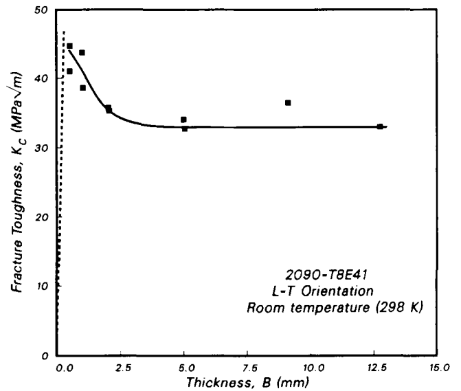
Fig. 11—Variation in Mode I fracture toughness K_c with test-piece thickness B for 2090-T8E41 alloy in the L-T orientation at 298 K. Tests were performed on C(T) specimens, machined from the plate mid-thickness, using anti-buckling restraints to prevent out-of-plane sliding.
