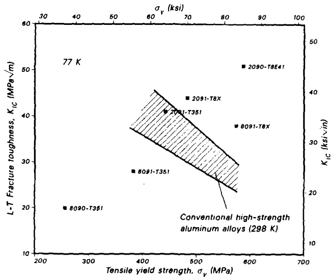
Fig. 4.—Combination of yield-strength and fracture-toughness properties for commercial aluminum-lithium alloys at liquid nitrogen temperatures, showing a comparison with ambient temperature data on typical aerospace high-strength aluminum alloys (hatched region after Ref. 22).
