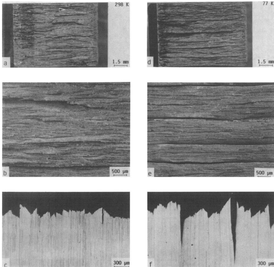
Fig. 7—Fractography and crack-path morphology for the L-T (crack-divider) orientation, typical of alloys which show no fracture-mode transition between ambient and liquid-nitrogen temperatures (2090-T8E41, 2091-T351, 8090-T8X, 8091-T8X), showing transgranular shear fracture at 298 K ((a), (b), and (c)) and 77 K ((d), (e), and (f)). Note how the degree of intergranular (short-transverse) delamination is enhanced significantly at liquid-nitrogen temperatures. Fracture surfaces are for 2090-T8E41. Arrow indicates general direction of crack growth.
