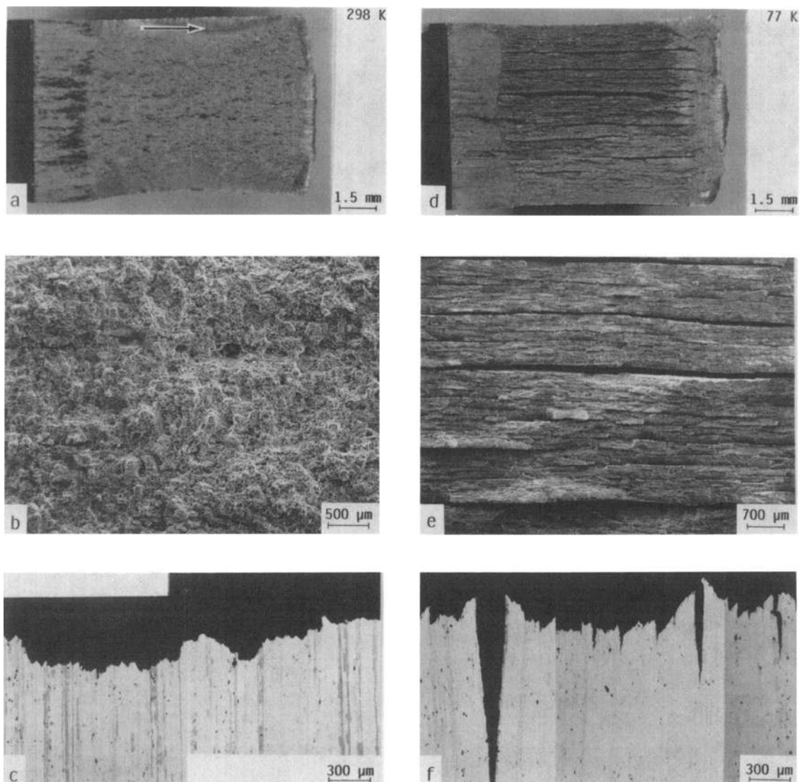
Fig. 6- Fractography and crack-path morphology for the L-T (crack-divider) orientation, typical of alloys which show a fracture-mode transition between ambient and liquid-nitrogen temperatures (2091-T8X, 8090-T351, 8091-T351), showing ductile microvoid coalescence at 298 K ((a), (b), and (c)) and transgranular shear fracture at 77 K ((d), (e), and (f)). Note the presence of intergranular (short-transverse) delaminations at 77 K. Fracture surfaces are for 2091-T8X. Arrow indicates general direction of crack growth.
