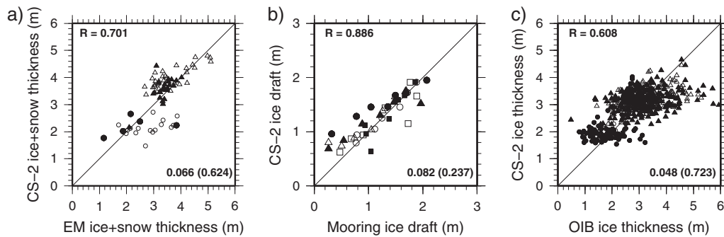
Figure 2. Validation of CryoSat sea ice thickness. (a) Comparison of Polar-5 aircraft EM and Cryosat-2 snow plus ice thickness over first year ( circle ) and multiyear (triangle) ice during April 2011 (open symbols) and 2012 (solid symbols). (b) Comparison of monthly average ice draft from CryoSat-2 within 200 km of the Beaufort Gyre Experiment Program Upward Looking Sonar Moorings (Mooring A: triangle, Mooring B: circle, Mooring D: square) for the period October 2010 to April 2011 and October 2011 to April 2012 (solid symbols). (c) Comparison of Operation IceBridge (OIB) aircraft laser and Cryosat-2 ice thicknesses over first year ( circle ) and multiyear (triangle) ice between 10 March 2011/12 and 9 April 2011/12 (solid symbols are data from 2012). Both aircraft comparisons were conducted by gridding CryoSat and the aircraft data onto a common (0.4 latitude by 4 longitude) grid and comparing those grid cells in which both data sets contained data. The locations of the in situ data sets are shown in Figure 1.
