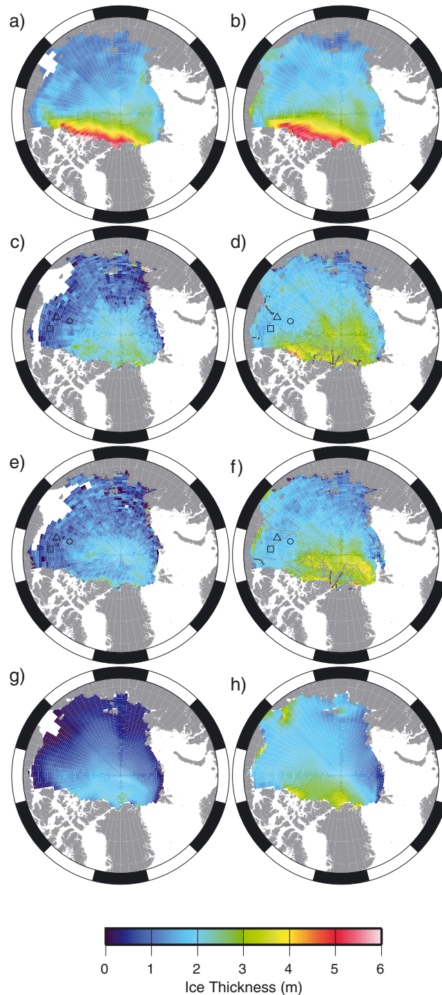
Figure 1. CryoSat sea ice thickness compared with PIOMAS and ICESat ice thickness measurements. The data are restricted to the “ICESat” domain covering the central Arctic Ocean. (a) 2003–7 average ICESat ice thickness for October/November and (b) 2004–8 average for February/March. (c and d) CryoSat thickness for October/November 2010 and February/March 2011 and locations of the airborne EM data (black lines) and OIB data (grey lines) used for validation, ULS moorings (triangle, circle, square). (e and f) CryoSat thickness for October/November 2011 and February/March 2012 and locations of the airborne EM data (black lines) and OIB data (grey lines) used for validation. (g) PIOMAS for October/November 2011 and (h) February/March 2012.
