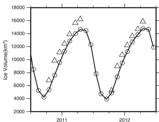
Figure 3. Timeseries of monthly Arctic sea ice volume from CS-2 (triangle) and from PIOMAS (solid line and circle) for two winter growth periods (October–April).
