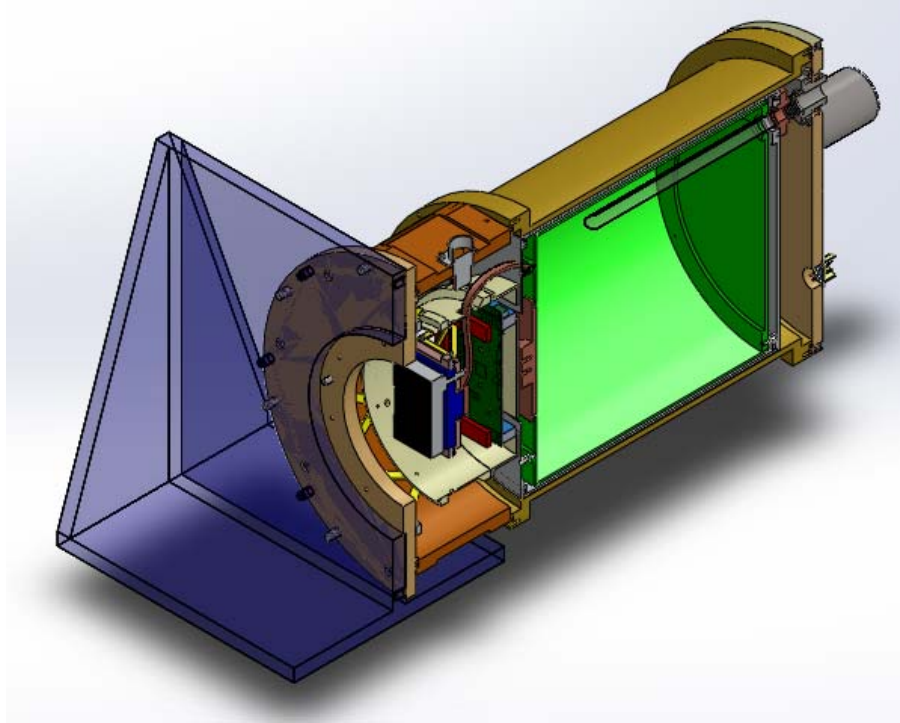
Figure 1. LN2 cryostat main body and CCD head support 3D model (cross section view). The right side of the image shows the vacuum jacket containing in the inside the LN2 tank and its filling tube; on the left side is the CCD head which contains the CCD, its mountings, copper strap, G10 supports, and PCB for electronics.
