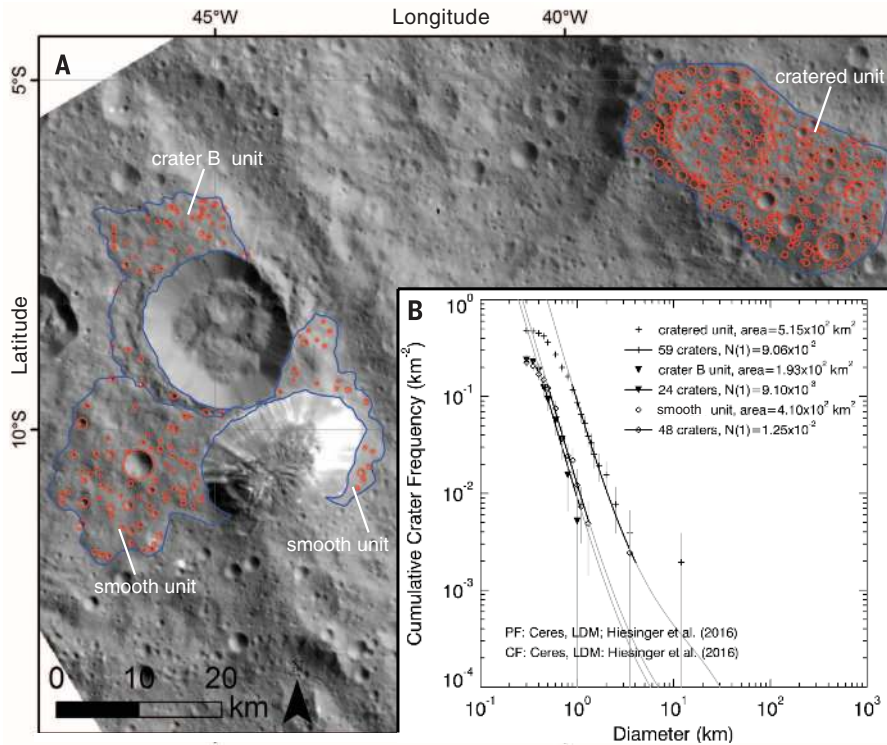
Fig. 5. Crater size-frequency distribution measurements of three areas in the Ahuna Mons region.
