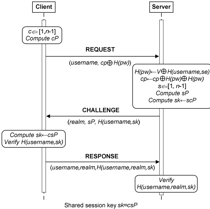
Fig. 2. Yoon's SIP authentication scheme
