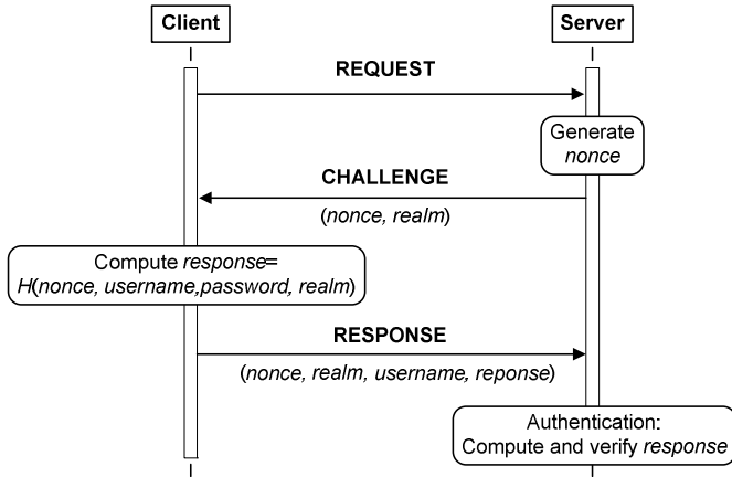
Fig. 1. SIP Authentication Procedure
