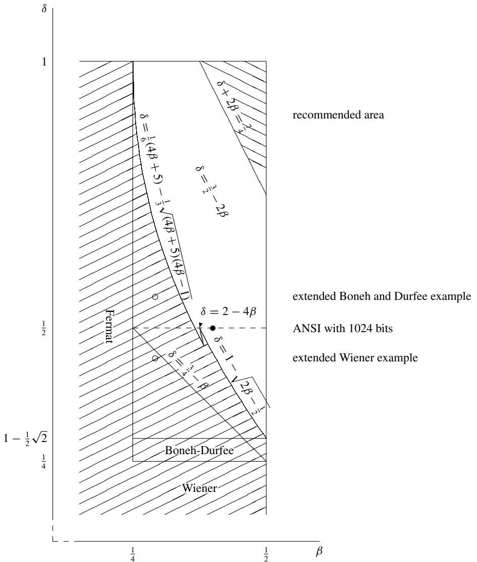
Fig. 1. Regions for \beta and \delta for which RSA is shown to be insecure.
