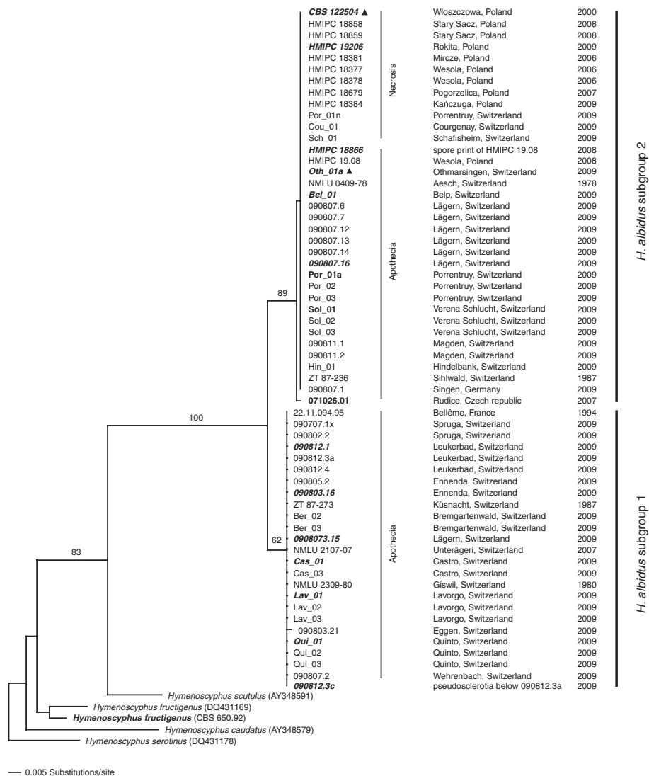
Fig. 1. Phylogenetic relationships within Hymenoscyphus albidus and among other Hymenoscyphus species based on DNA sequences of the ITS regions. Strains selected for genotyping (bold; see Fig. 2), type specimens (▲).
