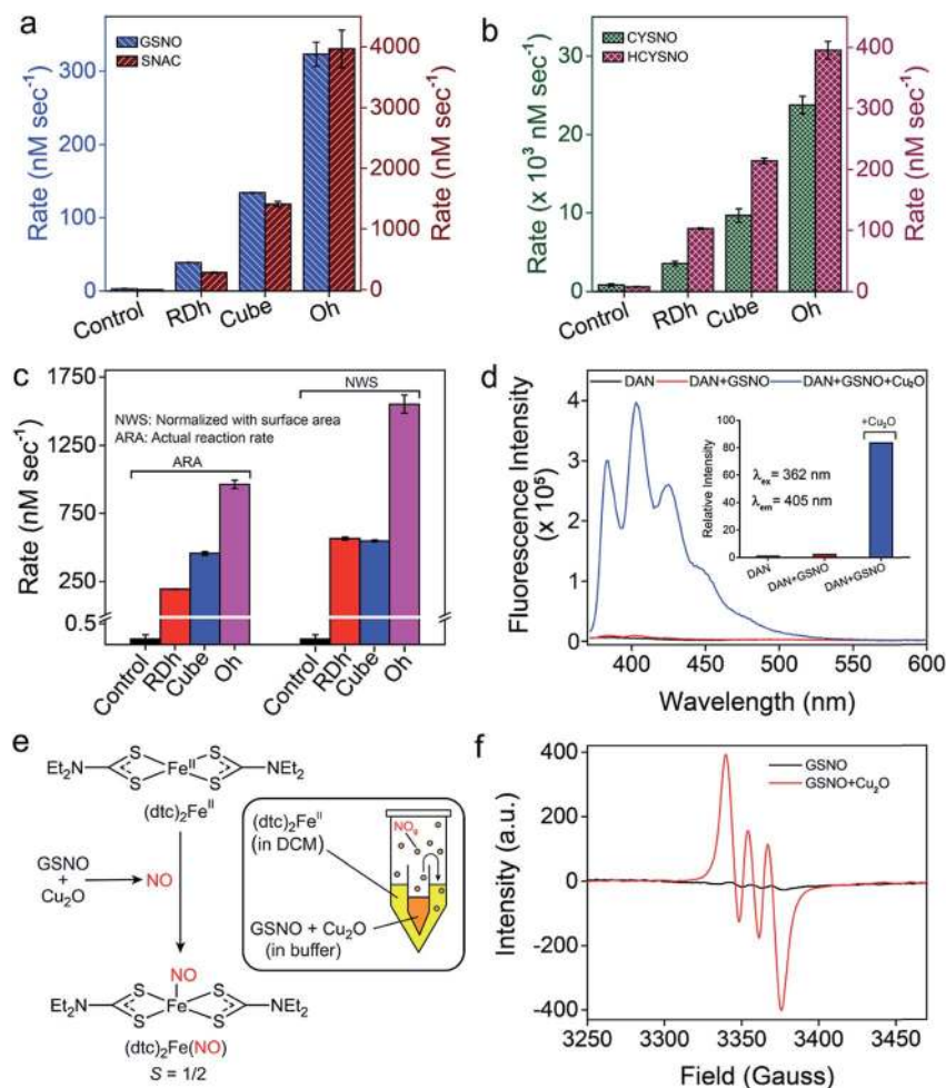
Fig. 3 (a and b) A comparison of the rate of denitrosylation by three different \text{Cu}_2\text{O} nanomaterials. (c) The actual rates of denitrosylation of SNAP ( 500 \mu\text{M} ) in the presence 2 \text{ ng } \mu\text{L}^{-1} of \text{Cu}_2\text{O} and a comparison with the rates obtained by normalizing the concentration with respect to 10 \text{ mm}^2 of the surface area. Assay conditions: 0.1 \text{ M} sodium phosphate buffer ( \text{pH } 7.4 ) at 25^\circ \text{C} . (d) Detection of NO by a fluorescence assay using DAN ( 5 \mu\text{M} ). (e) The reaction of (\text{dtc})_2\text{Fe} with NO generated from the reaction of GSNO with \text{Cu}_2\text{O} . (f) Room temperature electron paramagnetic resonance (EPR) spectra of [(\text{dtc})_2\text{FeNO}] complex.
