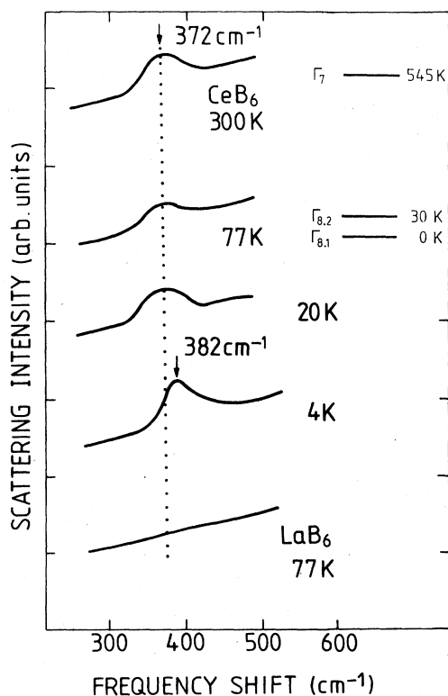
FIG. 2. Raman scattering intensities of \text{CeB}_6 and \text{LaB}_6 at different temperatures showing the \text{Ce}^{3+} \Gamma_8\text{-}\Gamma_7 CEF transition. Inset: Derived CEF level scheme of \text{CeB}_6 .
