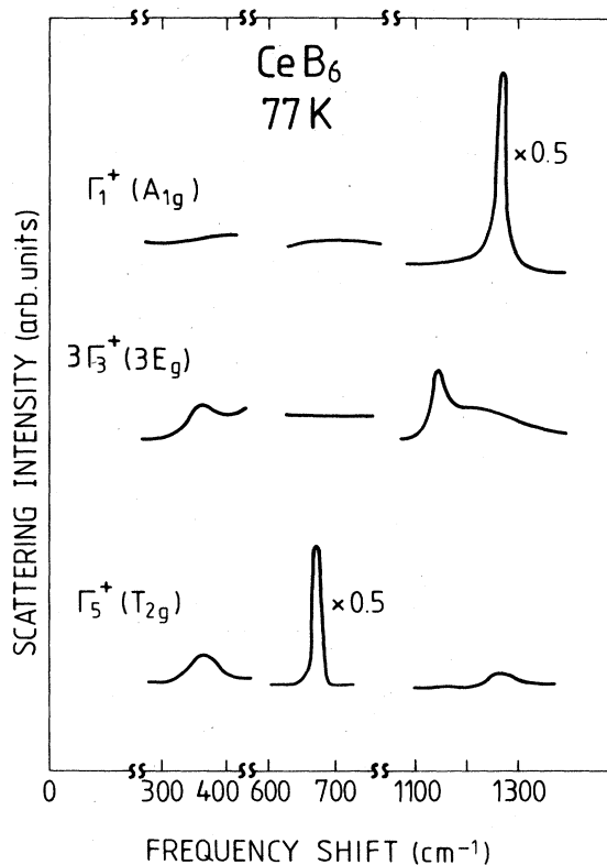
FIG. 3. Symmetry analysis of the \Gamma_8\text{-}\Gamma_7 CEF transition and the Raman-active phonons of \text{CeB}_6 .
