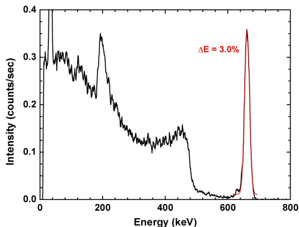
Fig. 4. Pulse height spectrum of SrI 2 :5% Eu under 137 Cs gamma ray excitation using a shaping time of 4 μs.
