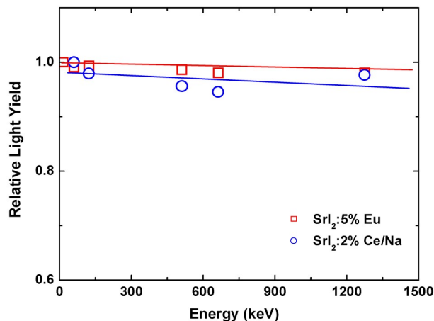
Fig. 5. Light yield proportionality as function of gamma ray energy of SrI 2 :5% Eu and SrI 2 :2% Ce/Na.
