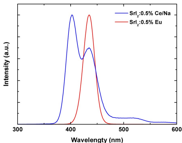
Fig. 2. Radioluminescence spectrum of \text{SrI}_2:0.5\% \text{Eu} and \text{SrI}_2:0.5\% \text{Ce/Na} .
