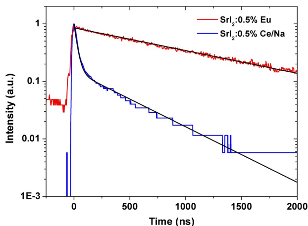
Fig. 3. Scintillation decay time spectra of \text{SrI}_2:0.5\% \text{Eu} and \text{SrI}_2:0.5\% \text{Ce/Na} under ^{137}\text{Cs} gamma ray excitation.
