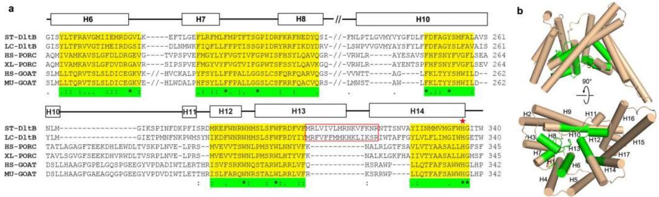
Figure 4 | Conserved regions among bacterial DltB and vertebrate Porcine/GOAT proteins. a , Alignment of conserved regions of DltB, Porcine (PORC) and GOAT. Conserved sequences are highlighted in yellow (and in green under the sequences). The red rectangle indicates the DltB-specific insertion, which is involved in the binding of DltC(Ppant). A red star marks the most conserved histidine residue among MBOATs. Abbreviations: Streptococcus thermophilus (ST), Lactobacillus casei (LC), Homo sapiens (HS), Xenopus laevis (XL), Mus musculus (MU). b , Conserved MBOAT core. Conserved regions among MBOATs form a central core in DltB structure (colored in green), whereas the peripheral helices shielding the core are largely non-conserved (colored in wheat).
