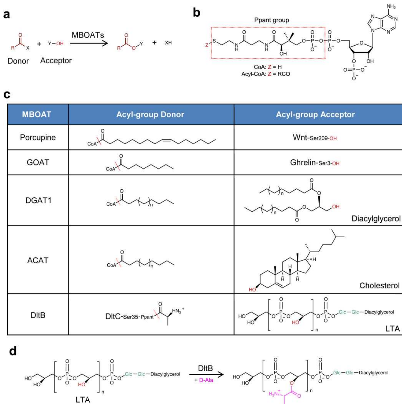
Extended Data Figure 1 | MBOAT catalyzed reactions and chemical structures of MBOAT substrates.
