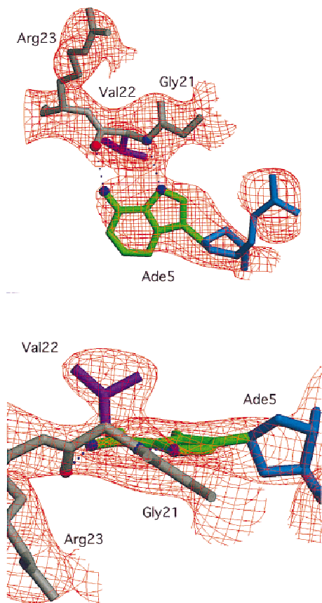
Figure 2. Electron density for the interaction between the adenine at the fifth position of the octamer element and Val-22. An SA-omit electron density map (which gives an unbiased way of checking a structure) was calculated with \sigma^A -weighted 2Fo-Fc coefficients (Read 1986) after omitting both Val-22 and the entire Ade-5 nucleotide from the final model and subjecting this partial model to simulated annealing in XPLOR (Brunger 1996). Gly-21 (gray), Val-22 (gray and purple), Arg-23 (gray), and Ade-5 (green and blue) from the final model are shown in the context of the SA-omit electron density contoured at 1.5\sigma . (A) The view perpendicular to the plane of the Ade-5 base (green, same view direction as in Fig. 3C) illustrates the electron density for the pair of hydrogen bonds (dotted lines) between the polypeptide backbone of Val-22 and the adenine ring. (B) The view looking into the major groove of the octamer element (same view direction as in Fig. 3A) illustrates the electron density for the Val-22 side chain (purple).
