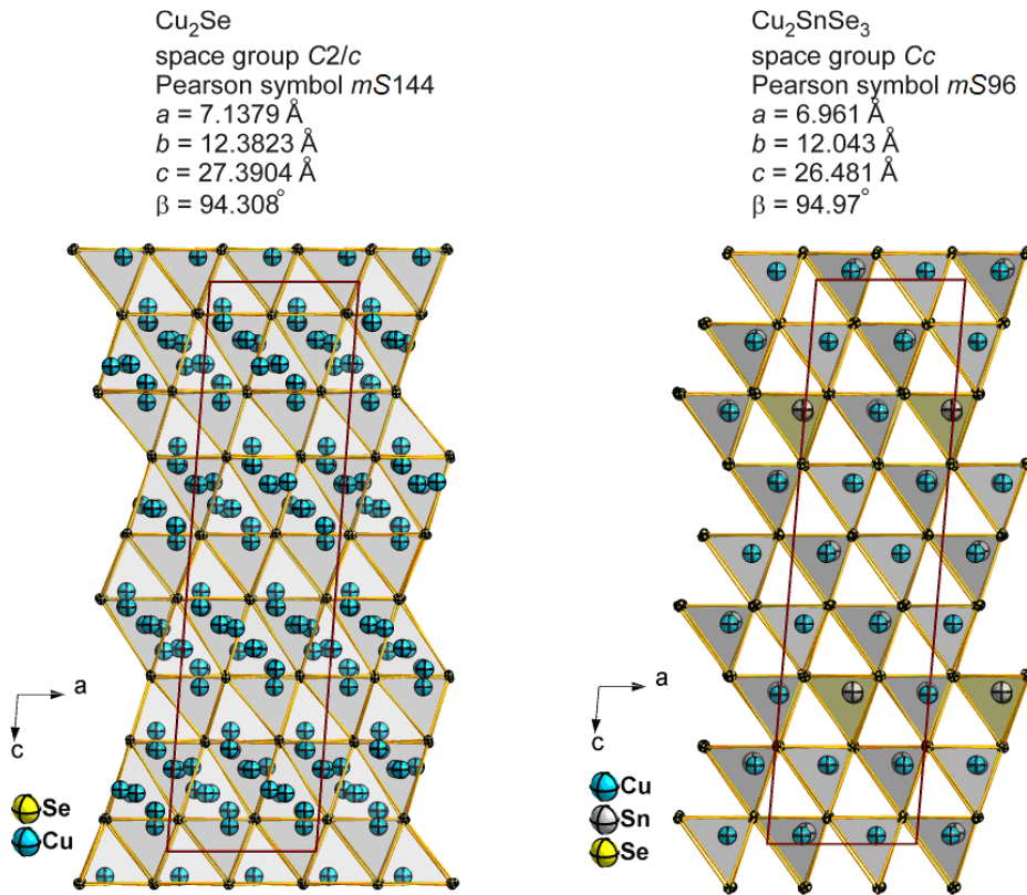
Fig. 4 Arrangement of Se tetrahedra and Cu and Sn atoms in the structures of LT-Cu 2 Se and Cu 2 SnSe 3 .
