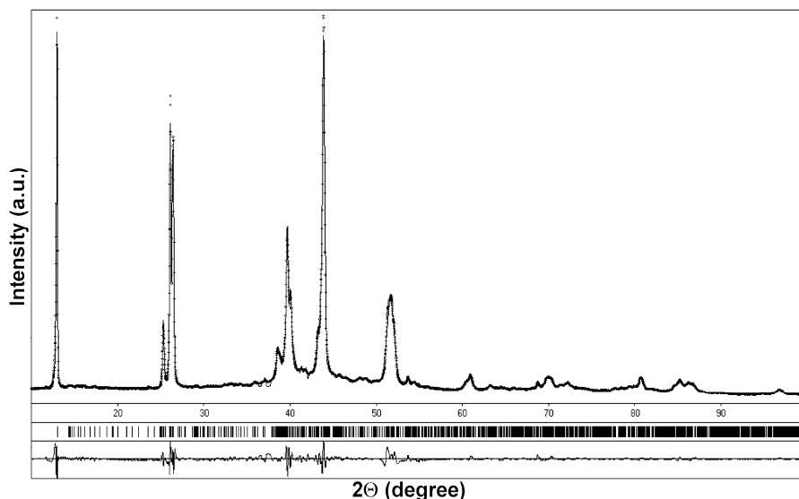
Fig. 1 Experimental and calculated diffractograms and the corresponding difference diagram for LT-Cu 2 Se.
