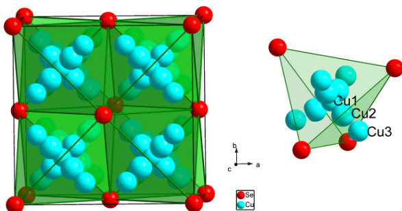
Fig. 5 Unit cell content and arrangement of Cu atoms in/near one Se 4 tetrahedron in HT-Cu 2 Se.
