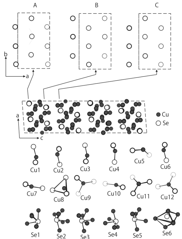
Fig. 3 Unit cell content and coordination polyhedra for LT-Cu 2 Se.
