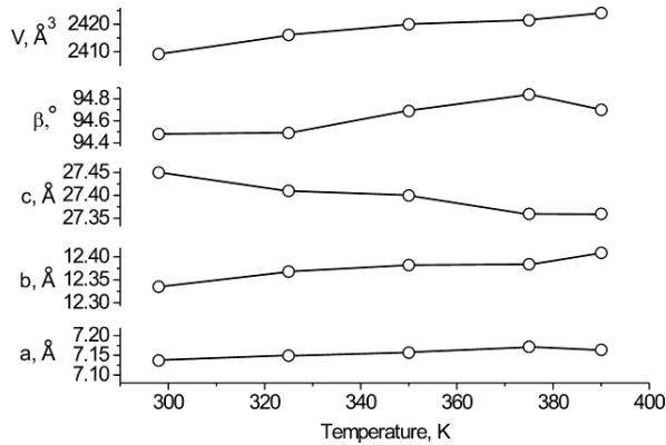
Fig. 2 Variation of the lattice parameters with temperature for LT-Cu 2 Se.
