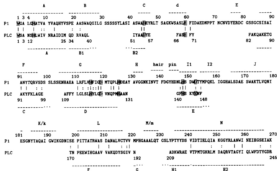
Fig. 8. The complete amino acid sequence of P1 and an alignment of those 145 residues of B. cereus phospholipase C (sequenced by Johansen et al. , 1988) for which the X-ray structure (determined by Hough et al. , 1989) may be superimposed on the P1 model with a r.m.s. deviation of 1.8 Å. All Zn ligands are boxed. Sequence identities are highlighted by a vertical bar, conservative substitutions by a colon. Secondary structure elements of P1 and PLC are indicated above and below the sequence, respectively, using capital letters for the labeling of \alpha -helices and small letters for 3_{10} -helices.
