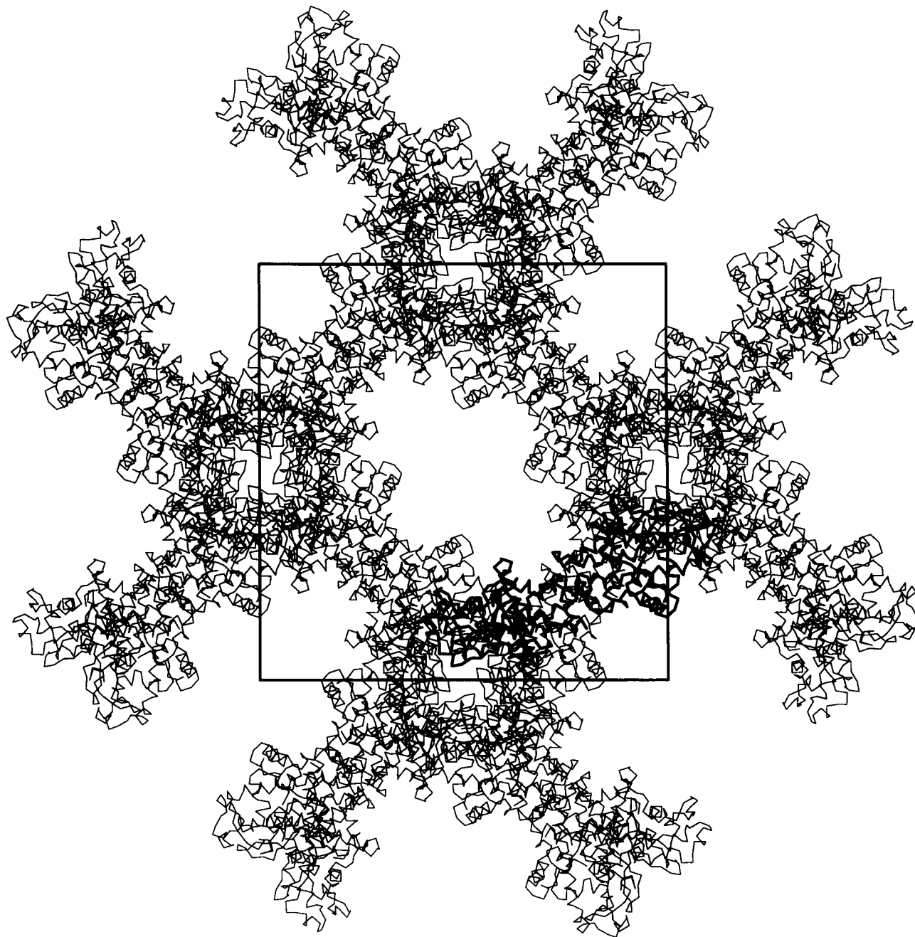
Fig. 6. Packing diagram for the tetragonal crystal form of P1, viewed along the four-fold screw axis. The square box shows the a and b unit cell edges. P1 molecules are represented by their C_{\alpha} traces. One non-crystallographic dimer is indicated in heavy lines.
