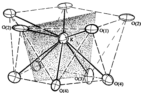
Fig. 4. Coordination of the \text{K}^+ ion in potassium pentavanadate. The intersection of the crystallographic mirror plane is shown shaded. The dashed lines show the pentagonal antiprismatic coordination.
