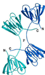
Dimeric \beta 2 -crystallin
