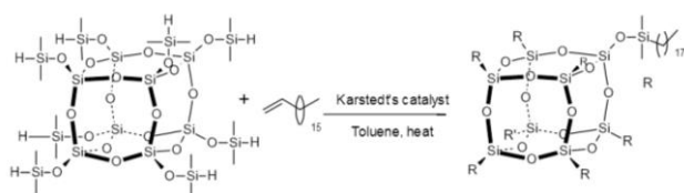
Figure 2. General synthetic route for the Q 8 C 18 POSS cage system 16 .
