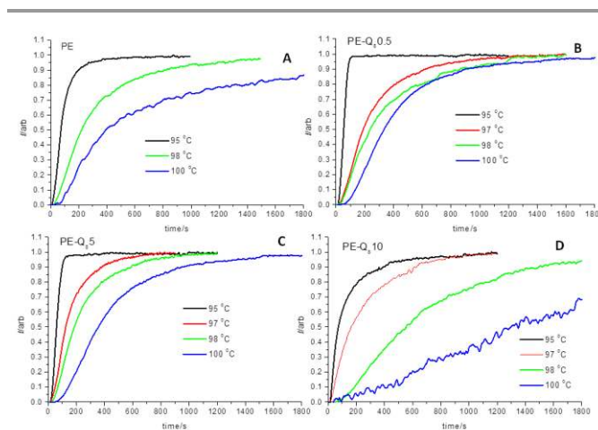
Figure 6. Isothermal crystallization curves at several temperatures for pure PE and selected blends from the time-resolved SAXS invariant data. (A) Pure PE; (B) PE-Q 8.5 blend; (C) PE-Q 8.5 blend; (D) PE-Q 8.10 blend.
