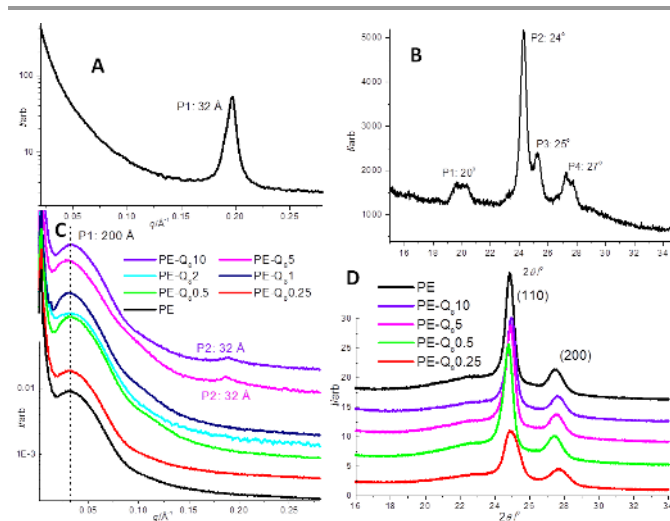
Figure 4. Static SAXS and XRD scans for pure PE and PE-POSS blends at 25 °C. (A): SAXS of pure Q 8 C 18 POSS; (B): XRD of pure Q 8 C 18 POSS; (C): SAXS of pure PE and PE-POSS blends; (D) XRD of pure PE and selected PE-POSS blends. Data in all plots are vertically off-set for clarity.
