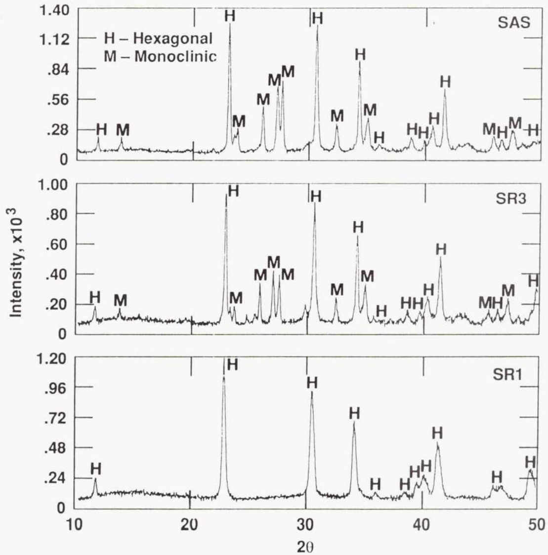
Figure 5.—Powder x-ray diffraction patterns of cold isostatically pressed and sintered (900 °C, 20 hr) glass powders of three different compositions in the (\text{Sr, Ba})\text{O} \cdot \text{Al}_2\text{O}_3 \cdot 2\text{SiO}_2 system.
