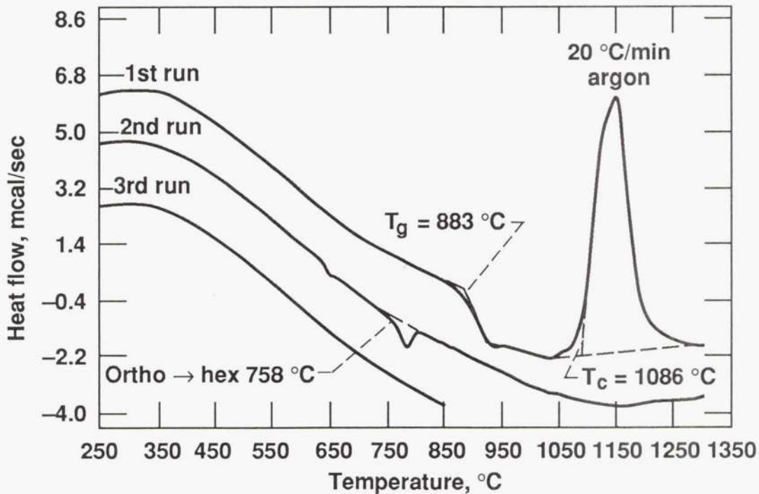
Figure 2.—Repeated DSC scans of bulk SAS glass. T_g is the glass transition temperature and T_c is the crystallization onset temperature.
