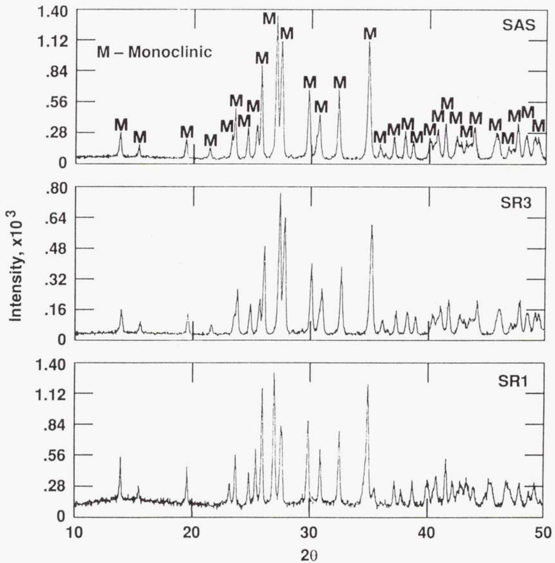
Figure 6.—Powder x-ray diffraction patterns of cold isostatically pressed and sintered (1100 °C, 20 hr) glass powders of three different compositions in the (\text{Sr, Ba})\text{O} \cdot \text{Al}_2\text{O}_3 \cdot 2\text{SiO}_2 system.
