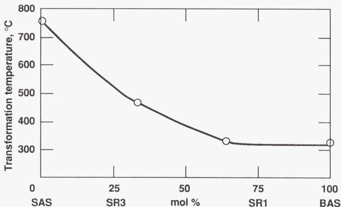
Figure 3.—Effect of composition on the orthorhombic to hexacelsian phase transformation temperature in the (\text{Sr}, \text{Ba})\text{O} \cdot \text{Al}_2\text{O}_3 \cdot 2\text{SiO}_2 system from DSC.
