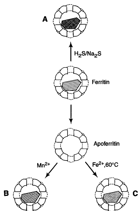
Fig. 7. The use of supramolecular protein cages (ferritin) in the synthesis of nanophase inorganic materials. The products are (A) iron sulfide, (B) manganese oxide, and (C) magnetite ( \text{Fe}_3\text{O}_4 ).
