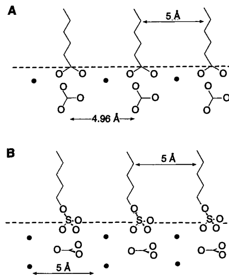
Fig. 4. Geometric and stereochemical complementarity at monolayer-crystal interfaces. (A) Nucleation of the calcite {1 \bar{1} 0} face under carboxylate monolayers. (B) Nucleation of the calcite {001} face under sulfate monolayers.
