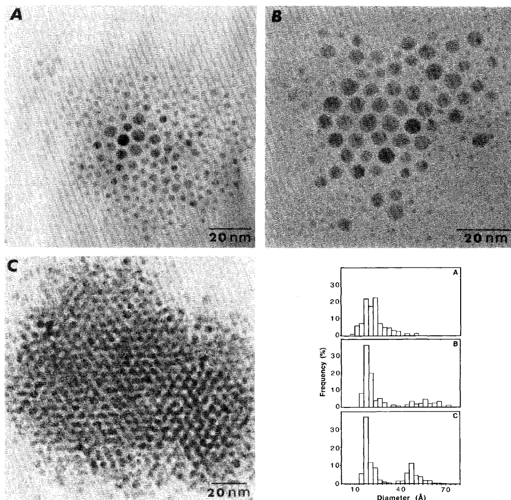
FIG. 1. TEM micrographs revealing the size-dependent phase separation and opal formation of weakly attracting alkylthiol-functionalized Au nanocrystals. Below (right) are the corresponding particle size distributions. As discussed in the text, only the largest particles (5–6 nm) attract each other sufficiently to order into closest packed domains. The transition from micrographs (a) to (b) shows the nucleation and 2D growth of such a domain. (c) A 3D hcp opal prepared by evaporating a hexane solution of particles on a water surface and lifting off the resulting Langmuir film onto a TEM grid.
