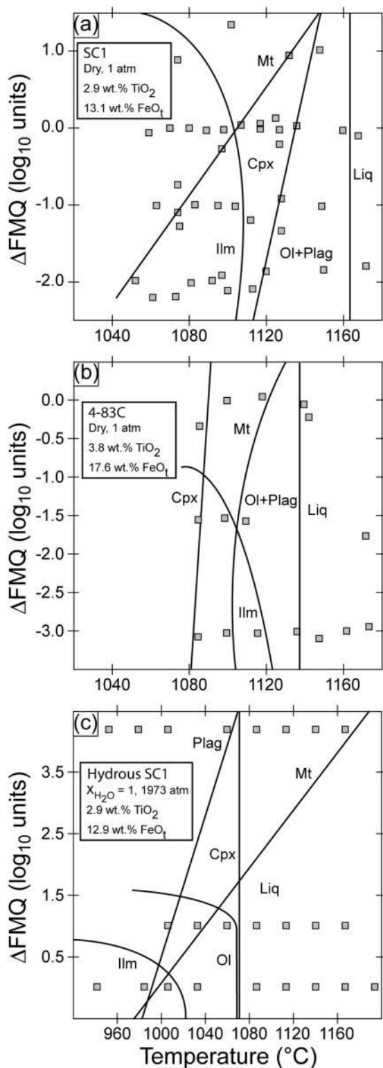
Fig. 12. Experimentally determined phase equilibria in ferrobasic melts as a function of oxygen fugacity and temperature. (a) Phase equilibria from 1 atm experiments on dry ferrobasic melt (SC1) with 13 wt % \text{FeO}_t and 3 wt % \text{TiO}_2 from Toplis & Carroll (1995). (b) Phase equilibria from 1 atm experiments on dry ferrobasic melt (4-83C) with 18 wt % \text{FeO}_t and 4 wt % \text{TiO}_2 from Snyder et al. (1993). (c) Phase equilibria from 1970 atm experiments on hydrous ferrobasic melt (hydrous SC1) from Botcharnikov et al. (2008).
