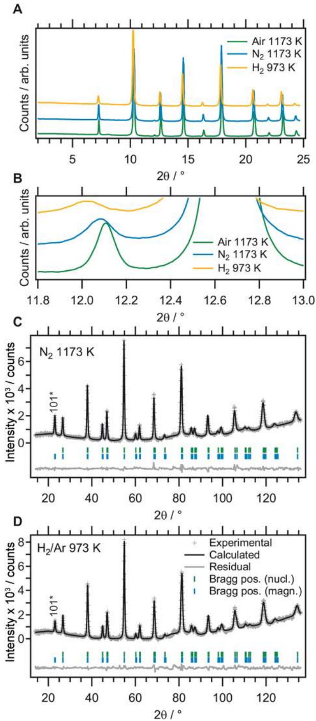
Fig. 9 (A) Synchrotron XRD patterns of the samples heated in air, nitrogen and hydrogen to 1173 K, 1173 K and 973 K, respectively. (B) Detailed view of the region around the rhombohedral (113) reflex, which is present in all specimens. The lower panels show the results of the structural refinement of neutron diffraction data of LSF heated in (C) N 2 to 1173 K and (D) H 2 /Ar to 973 K.
