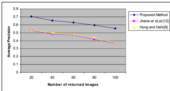
Fig. 7 The average precision of different methods
