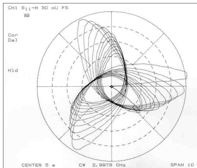
Figure 9.4 Bead-pull measurement: an error of about 40° between the 1 st and last cell is measured in this reflection diagram, corresponding to a phase slip of ±10° between electron and wave over 32 cells. The loss in accelerating efficiency is less than 1%. The cells are not equipped with dimple tuners.
