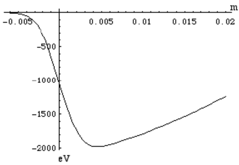
Figure 13.9 Distribution of the energy loss inside 2 mm Gaussian bunch with 2.33 nC charge.
