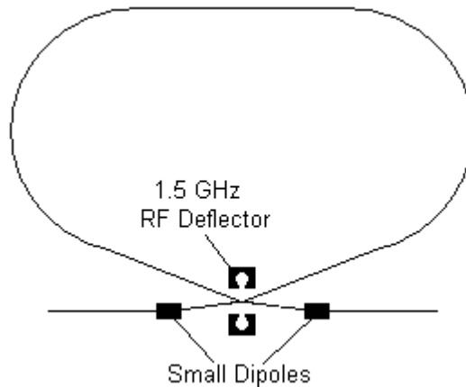
Figure 14.1 Delay Loop Injection Scheme.
