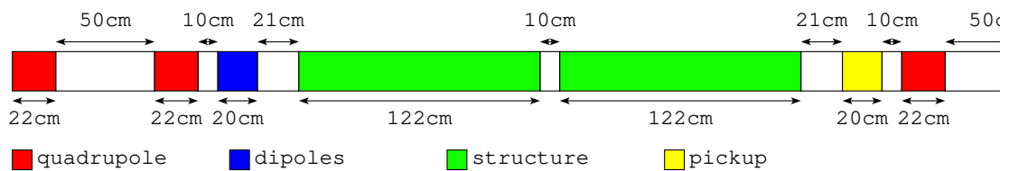
Figure 10.5 Sketch of a single cell in the doublet lattice.
