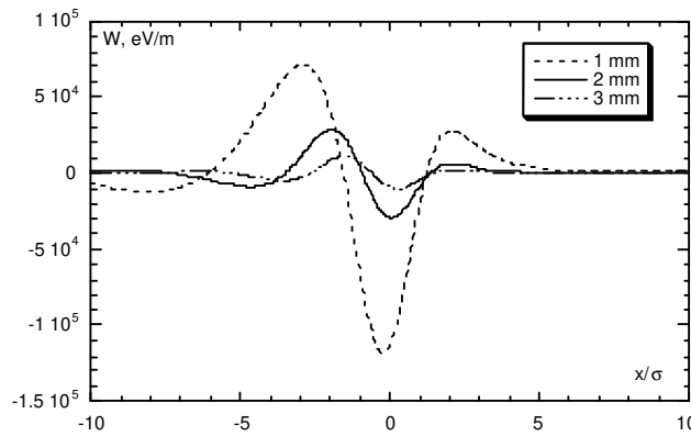
Figure 13.2 CSR wake force in EPA magnets for different bunch lengths.
