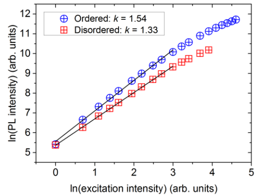
Figure 6 Dependence of RT- PL intensity on excitation intensity for ordered and disordered pieces of a \text{Cu}_2\text{ZnSnS}_4 sample. The straight lines indicate the regions of data from which the k -factors were calculated.
