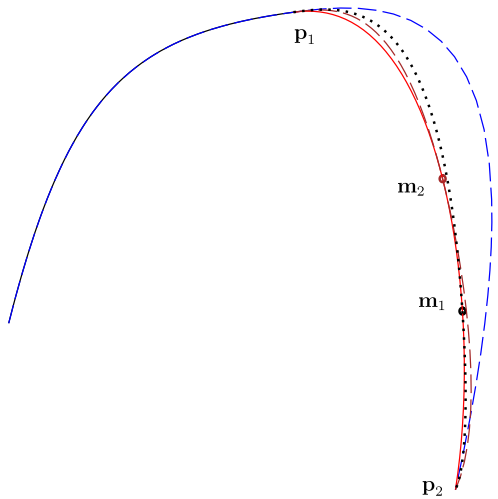
Fig. 9. The dotted segment in black and the dashed segment in brown are obtained by using inner points \mathbf{m}_1 and \mathbf{m}_2 , respectively. It can be verified that MSDA(\mathbf{m}_2) > MSDA(\mathbf{m}_1) , and the corresponding Hausdorff distance by using \mathbf{m}_2 is smaller.
