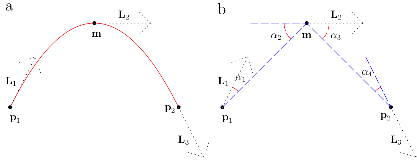
Fig. 8. Illustration of the minimum shape deformation angle of an inner point \mathbf{m} between \mathbf{p}_1 and \mathbf{p}_2 : (a) three points and their derivative vectors; and (b) the minimum shape deformation angle of the inner point \mathbf{m} .
