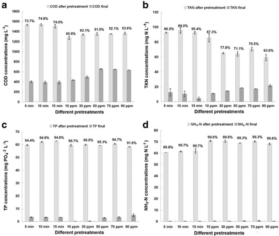
Fig. 1 Characteristics of the dairy wastewater before and after 4-day cultivation ( a , b , c , d refer to COD, TKN, TP, NH 3 -N, respectively). The values above the columns refer to the removal rate of each pretreatment
