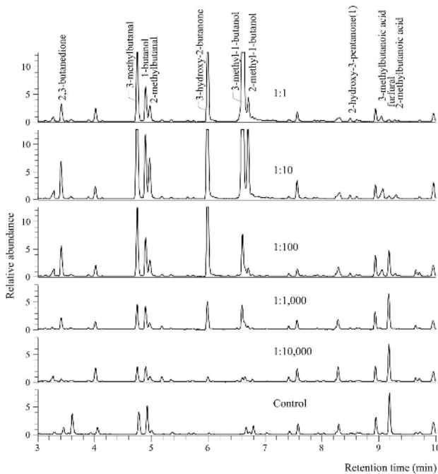
Figure 5 GC-MS chromatogram of headspace samples of skin microbiota. Part of GC-MS chromatograms of headspace samples of blood agar plates with different dilutions of skin microbiota and a blood agar plate without skin microbiota showing 11 compounds that were present in significantly higher or lower amounts in the control (Table 3). All compounds were identified on the basis of matching spectra (NIST library), and verified by injection of a standard (except 2-hydroxy-3-pentanone).
