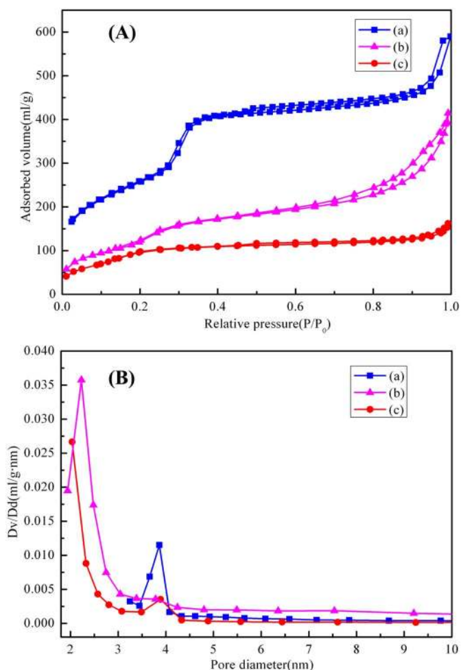
Figure 3 | Porous textures of the samples. (A) N_2 adsorption-desorption isotherms and (B) pore size distribution curves of the samples: (a) Al-MCM-41, (b) direct-synthesized CuO-Al-MCM-41 and (c) post-synthesized CuO-Al-MCM-41 respectively.
