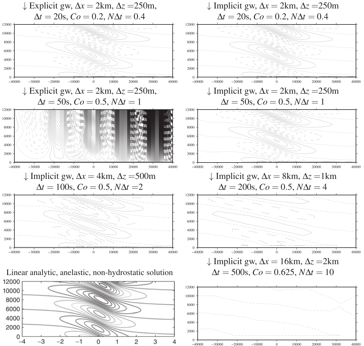
FIG. 7. Vertical velocity after 15000s for near-hydrostatic flow over a hill using the H model formulations with explicit and implicit gravity waves (gw) for different \Delta t , Co , and N\Delta t values. (bottom left) The analytic solution is taken from Fig. 4e in Melvin et al. (2010). Contours are 5 \times 10^{-4} \text{ m s}^{-1} , negative contours are dashed, and the zero contour is dotted.
