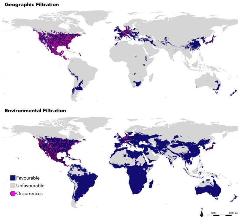
Figure 4. Projection of global bioclimatic favourable areas for Procyon lotor , predicted through Geographical Filtration and Environmental Filtrations approaches. Pink circles represent occurrences used in the modelling.
