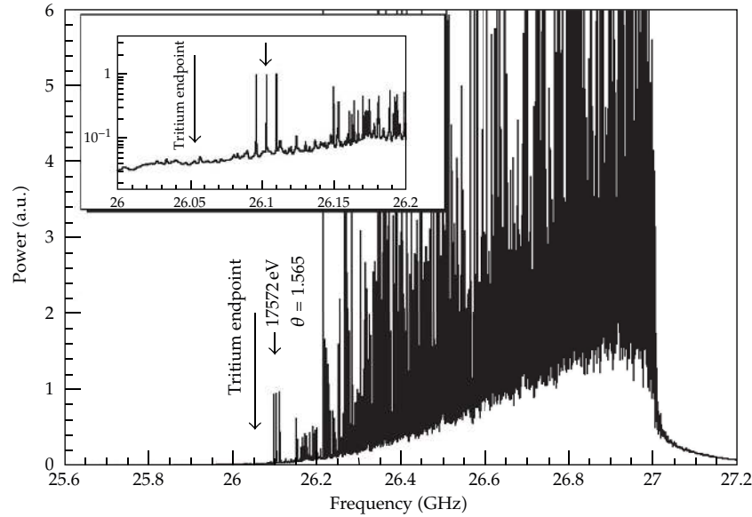
FIGURE 28: Simulated frequency spectrum of 10^5 tritium decays observed within a 30 \mu\text{s} interval in a 10 m long source with a field of 1 T. The inset shows the triplet of lines produced by a high energy electron (reprinted with permission from [170], Copyright (2009) by the American Physical Society).
