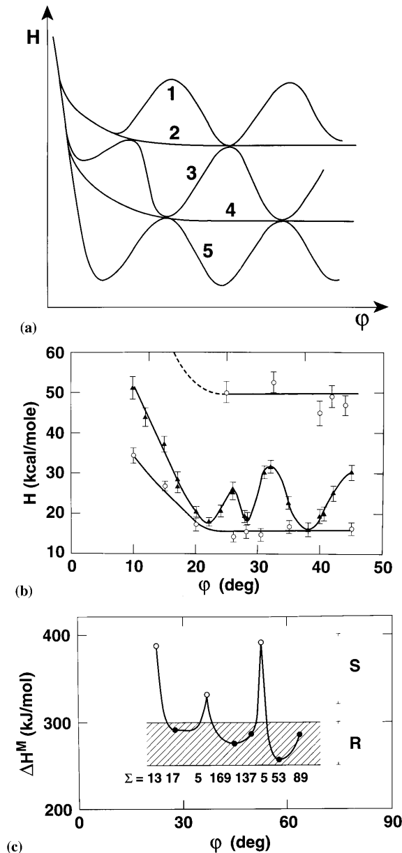
Fig. 43. (a) Schematic dependence of activation energy for grain boundary mobility for different purity levels: (1) concentrated alloy, (2) low purity, (3) high purity, (4) ultra-high purity, and (5) completely pure. (b) Measured dependence of activation energy for grain boundary mobility for \langle 100 \rangle tilt boundaries in Al of different purity levels: \square 99.9995 at.%, \triangle 99.9992 at.%, \circ 99.98 at.% [342]. (c) Measured dependence of activation energy for grain boundary mobility for \langle 100 \rangle tilt boundaries in Fe-6at.%Si at different purity levels [343]. S and R refer to special and random grain boundaries, respectively.
