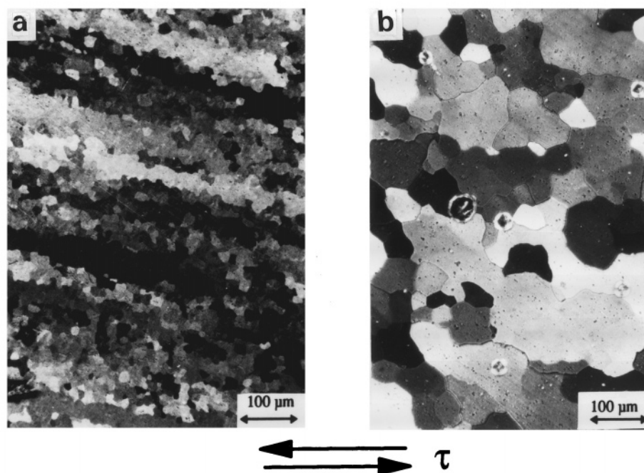
Fig. 34. Polarized optical micrographs of Al–5Mg in the solute drag regime showing substructure regions that may contain many subgrains as measured in TEM. (a) 400°C, 0.01 \text{ s}^{-1} , \varepsilon = 3.1 exhibits elongated grains with visible subgrains and serrations; (b) 500°C, 0.01 \text{ s}^{-1} , \varepsilon = 0.8 exhibits shortened grains with thickness of approximately the subgrain diameter as a result of GRX (a). the microstructure remains almost identical to this (in b) as the strain progresses to 3.4 without change in stress [231,240] (courtesy of R. Merkel).
