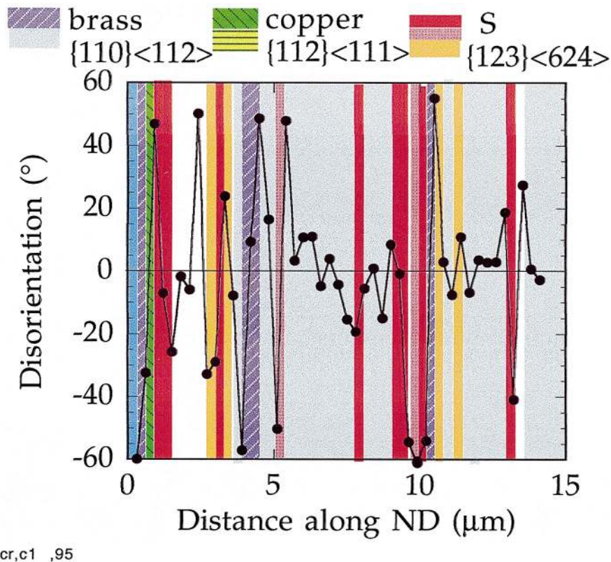
Fig. 7. The disorientation angles measured across dislocation boundaries in the normal direction for aluminum 90% cold rolled show an alternating character with distance. These boundaries separate finely distributed texture components as shown by the color shading.
