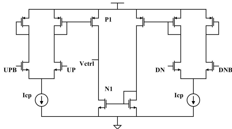
Figure 1. Conventional current-steering charge pump
