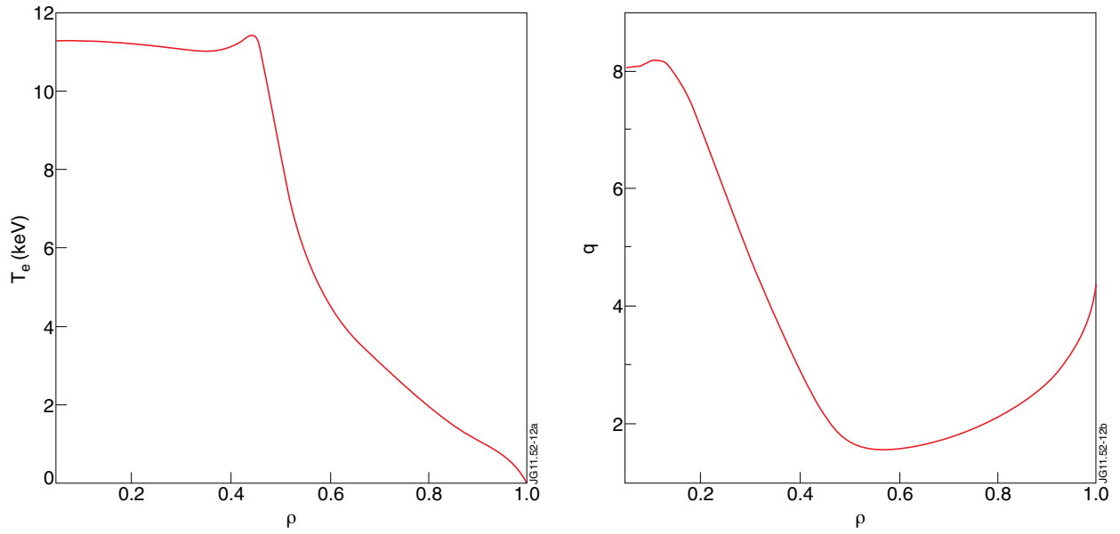
Figure 12: Projection of the ITER current ramp-up phase in case 20MW of ECRH are added at mid-radius early from t = 10s onwards (flat-top value I_p = 15MA reached at t = 70s ). The dynamic evolution of plasma expansion is solved by the TSC code with the CDBM transport model. Electron temperature (left) and q -profile (right) at the end of the current ramp.
