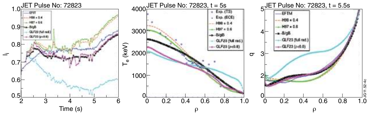
Figure 4 : Left : Simulation of the internal inductance dynamics of a JET LHCD assisted current ramp-up (2 MW of LHCD applied + 1.5MW NBI diagnostic beam) with several heat transport models. The plasma current is ramped up to 1.15MA in 5s. Same colour code as Fig.2. Middle : Electron temperature profile at t = 5s . Right : q -profile at t = 5.5s , with comparison to MSE constrained equilibrium reconstruction (blue, “EFTM”).
