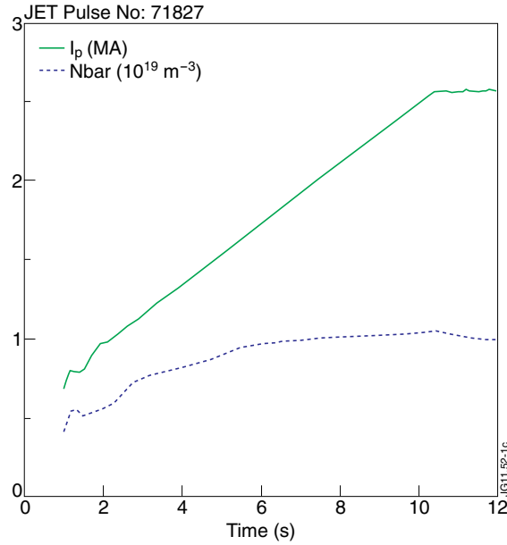
Figure 1 : Scenario of JET shot 71827 (ohmic). Time traces of plasma current I_p (green, solid) and central line averaged density N_{bar} (blue dots).
