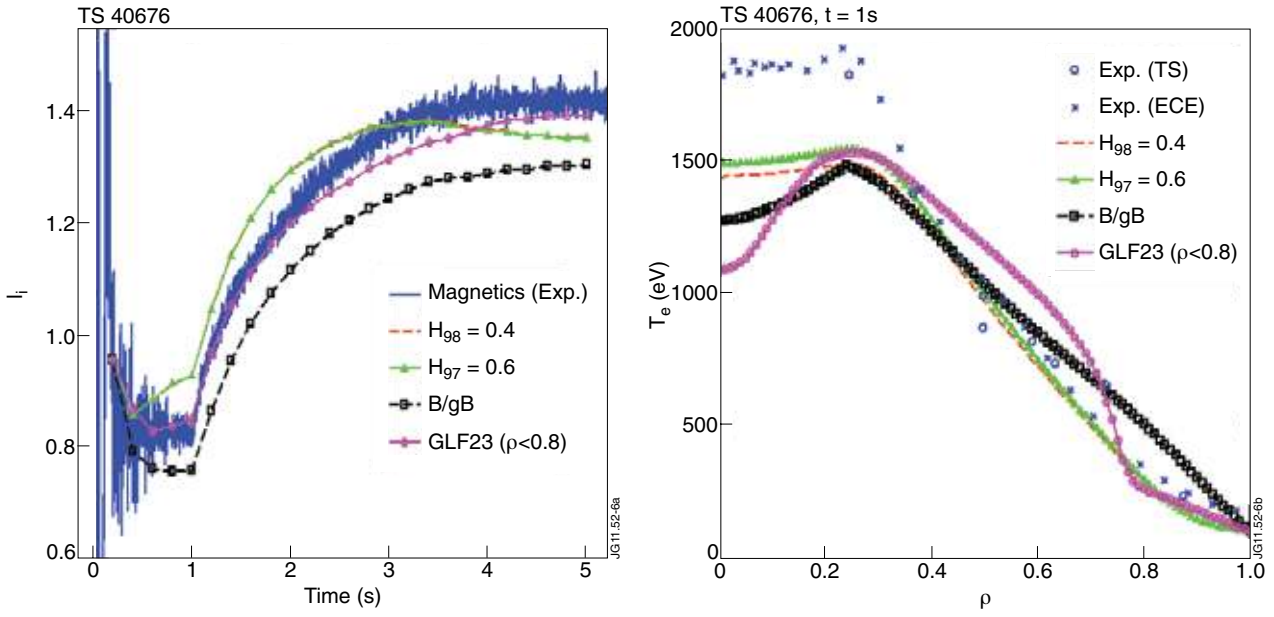
Figure 6 : Left : Simulation of the internal inductance dynamics of a Tore Supra ECCD assisted current ramp-up (co-ECCD applied at \rho = 0.3 ) with several heat transport models. The plasma current is ramped up to 0.9MA in 1s. Same colour code as Fig.2. Right : Electron temperature profile at t = 1 s.
