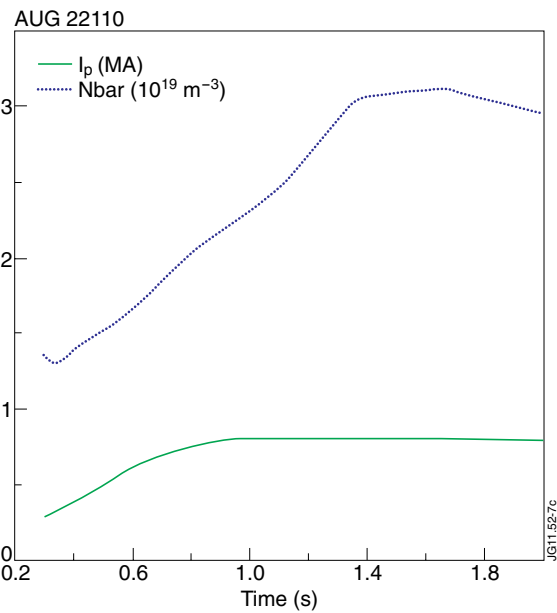
Figure 7 : Scenario of AUG shot 22110 (ohmic). Time traces of plasma current I_p (green, solid) and central line averaged density N_{bar} (blue dots).
