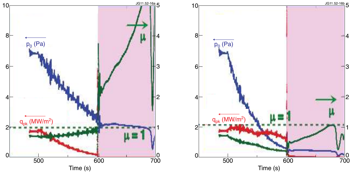
Figure 16: Left : Simulation of the divertor power load q_{pk} , the normalized neutral pressure \mu and the divertor neutral pressure p_0 , keeping the edge/core fuelling control invariant ( f_{edge/core} = 0.8 ). Right after H-L transition at 600sec, the operating point of inner divertor becomes strongly detached ( \mu \gg 1 ). Right : Simulation of q_{pk} , \mu and p_0 , changing f_{edge/core} from 0.8 at 500sec to 0 (totally core fuelling) at 600sec. Even after H-L transition, the operating point of inner divertor remains attached in “regime A” ( \mu < 1 ), though a higher heat pulse more than 10\text{MW/m}^2 arises at the H-L transition.
