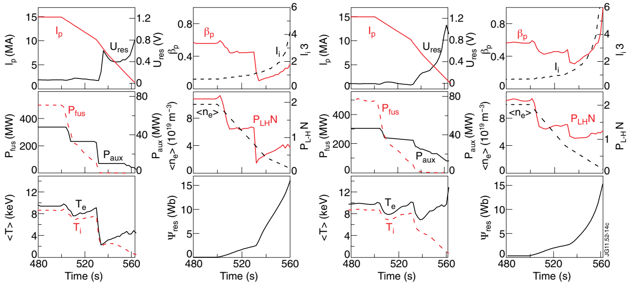
Figure 14: Plasma termination scenarios in L-mode (left, H-L transition triggered at t = 530 s by decreasing the additional power P_{aux} ), and staying in H-mode (right), simulated with the Astra code.
