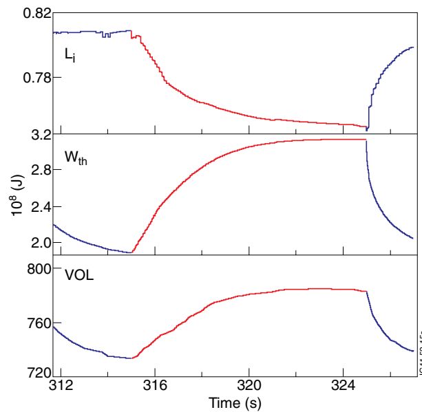
Figure 15. From top to bottom: internal inductance (plasma is in L-mode when colour is blue and in H-mode when colour is red), plasma thermal energy content and plasma volume
