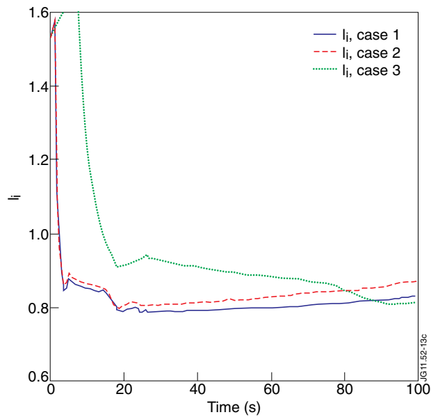
Figure 13: Sensitivity analysis in case of the ohmic ITER ramp-up case (flat-top value 15MA reached at t = 100s ) with the scaling-based model H_{98} = 0.4 . Case 1 (blue): constant Z_{eff} = 1.7 , T_{ea} ramped up from 25 to 250eV. Case 2 (red): constant Z_{eff} = 1.7 , T_{ea} 25-100eV. Case 3 (green): Z_{eff} ramped down from 4 to 1.7, T_{ea} 25-250eV.
