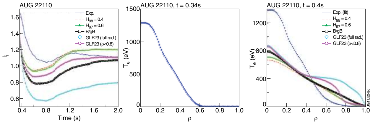
Figure 8 : Left : Simulation of the internal inductance dynamics of an AUG ohmic shot with several heat transport models. The plasma current is ramped up to 0.8MA in 0.9s. Same colour code as Fig.2. Middle : Electron temperature profile at t = 0.34s (fitted from measurements). Right : Electron temperature profile at t = 0.4s .
