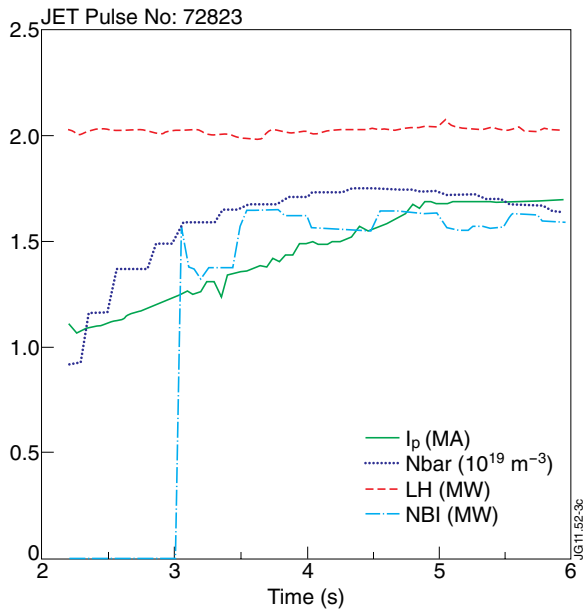
Figure 3: Scenario of JET Pulse No: 72823 (LHCD + NBI diagnostic beam). Time traces of plasma current I_p (green solid) central line averaged density N_{bar} (blue dots), LH power (red dash) and NBI (light blue dash dot).
