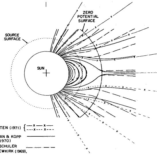
Figure 6. A comparison of solutions for a dipole solar field with the zero potential surface model [ Altschuler and Newkirk, 1969 ] the present model and the exact isothermal MHD coronal solution [ Pneuman and Kopp, 1970 ]. Note that the present solution is quite similar to the isothermal coronal solution supporting the suggestion that the coronal currents are confined to thin sheets.
